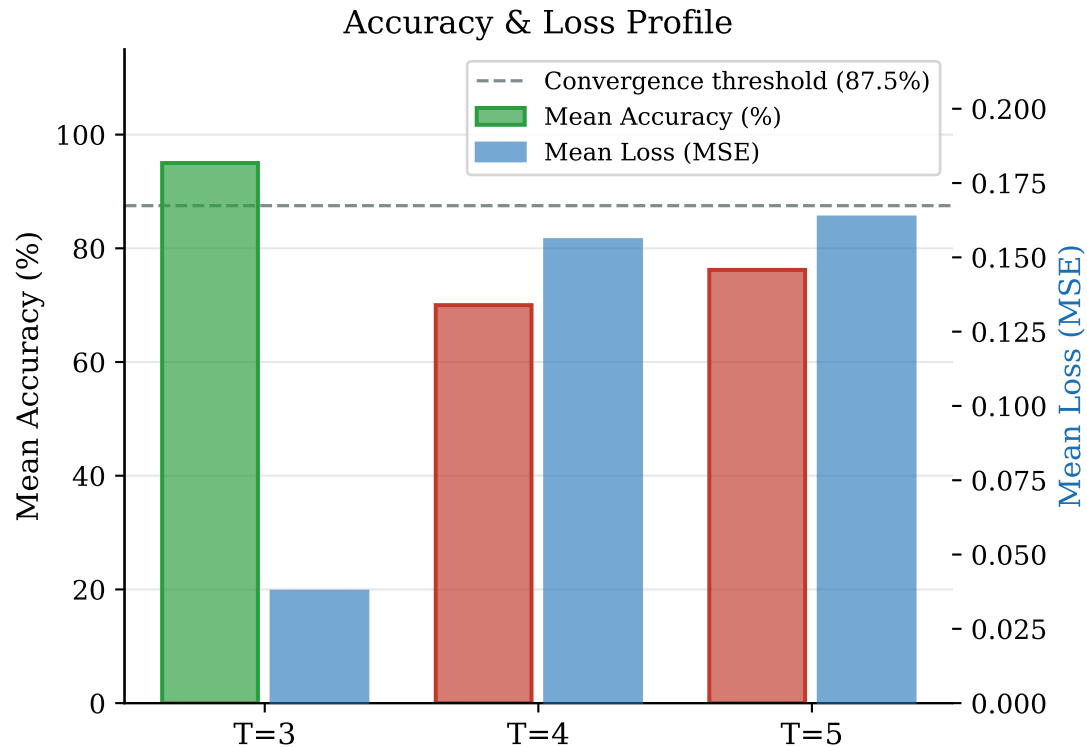
Figure 2: Archon's Discrete Trainability Cliff — 2-Qubit Q-RNN, Parity Task
