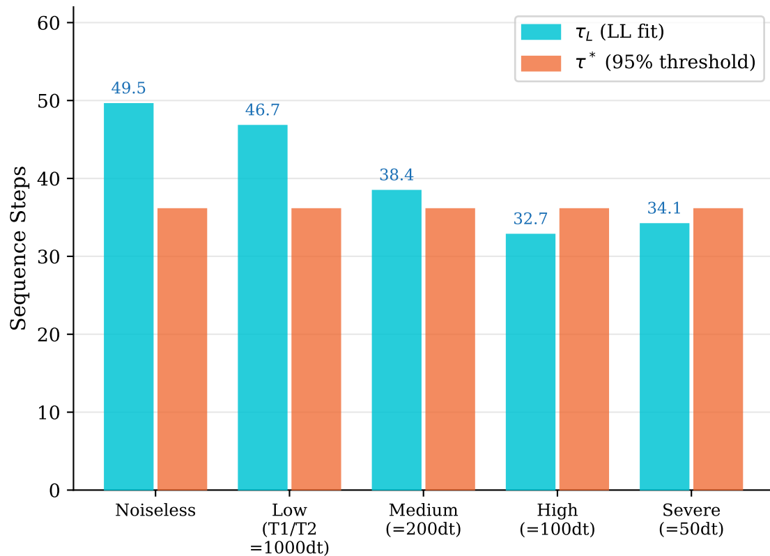
\tau_L and \tau^* vs Lindblad Noise
