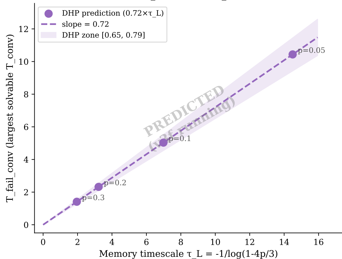
Figure 4: Memory-Qubit Noise Creates DHP (v3f)
