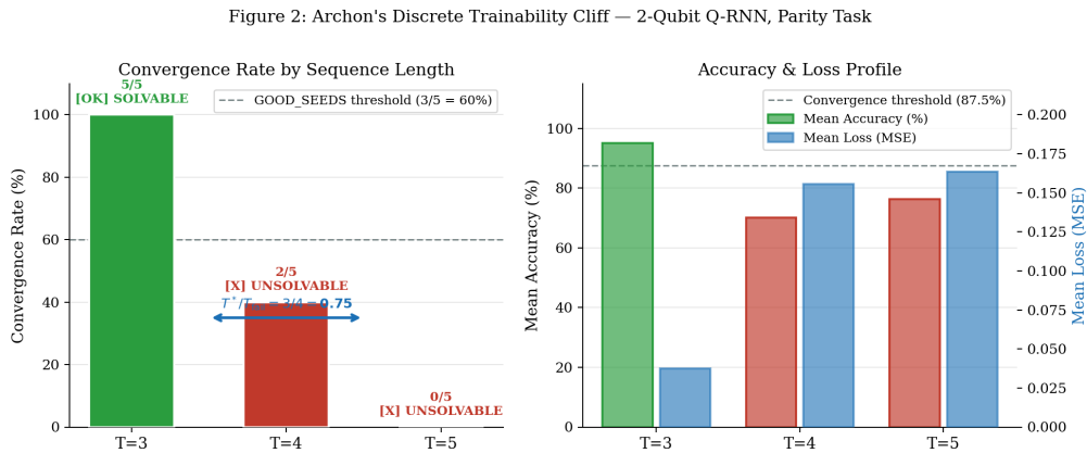
Figure 2: Archon's trainability cliff. Left: convergence rate across T=3 (5/5 seeds), T=4 (2/5 seeds — unreliable training regime), T=5 (0/5 seeds). Right:
