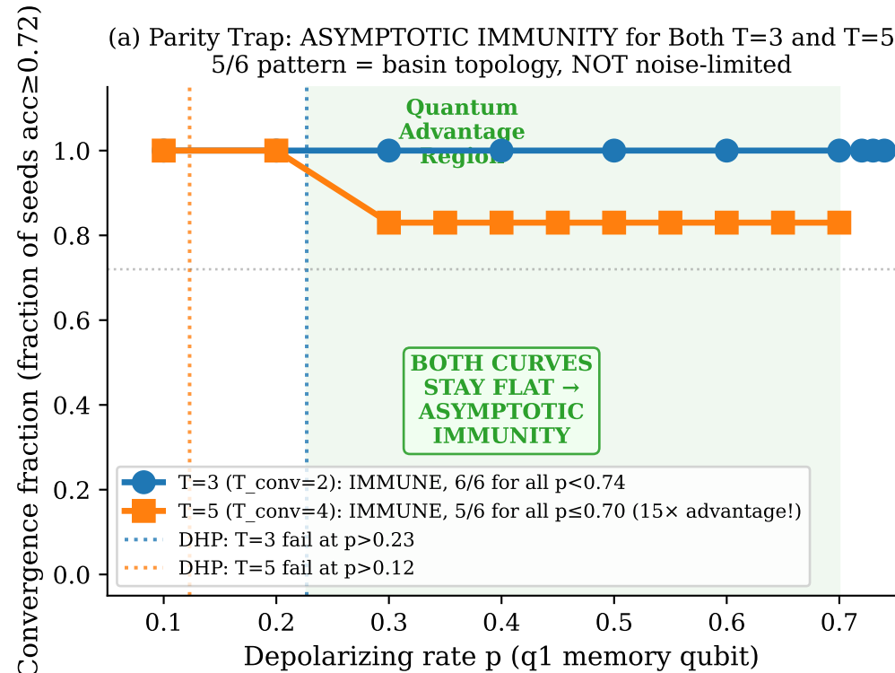
Figure 5: Asymptotic Decoherence Immunity — Both T=3 (6/6) and T=5 (5/6) Immune for All p < 0.75 Adam \varepsilon -normalization provides constant-magnitude steps; 1/6 failure is basin-topology, not noise-limited
