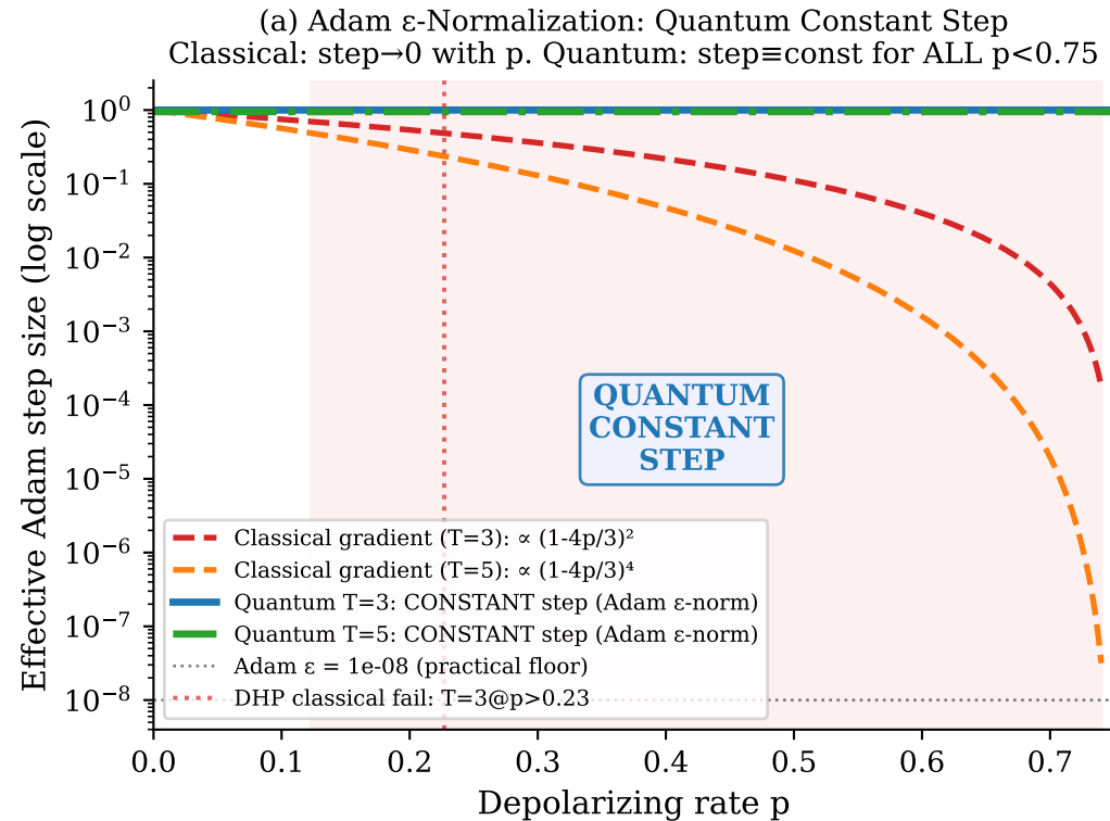
Figure 6: Asymptotic Quantum Advantage — Adam \varepsilon -Normalization Provides Immunity for All p < 0.75
