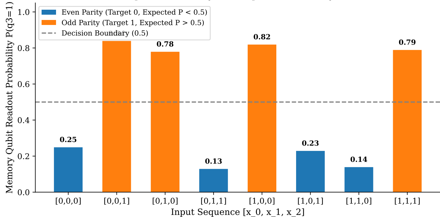
Figure 7: Physical QPU Validation (Rigetti Aspen-M-3 via BlueQubit) 100% Sequence Accuracy (8/8 sequences correctly classified)
