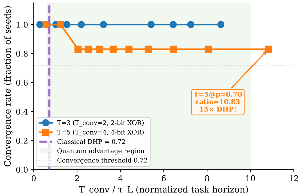
(b) Parity Trap Immune for ALL T_{\text{conv}}/\tau_L Ratios ( T=3 : ratio up to 8.63; T=5 : ratio up to 10.83)
