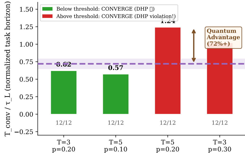
(a) Quantum vs Classical DHP Threshold Red bars: above DHP \rightarrow should fail but DON'T
