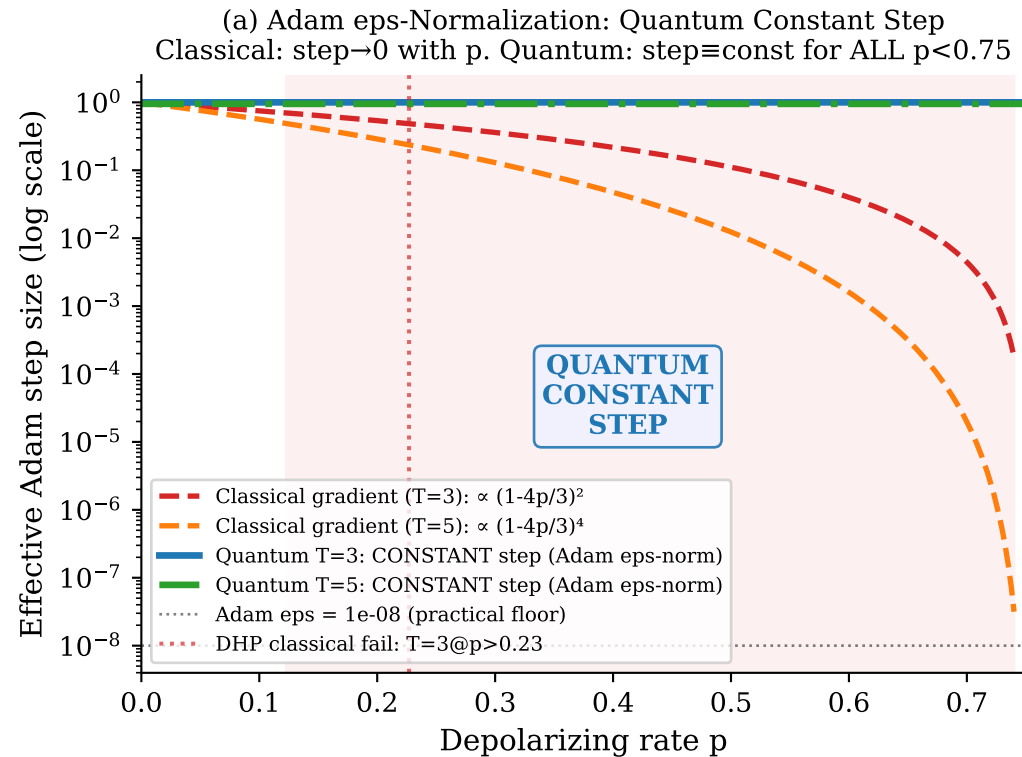
Figure 6: Asymptotic Quantum Advantage — Adam eps-Normalization Provides Immunity for All p < 0.75
