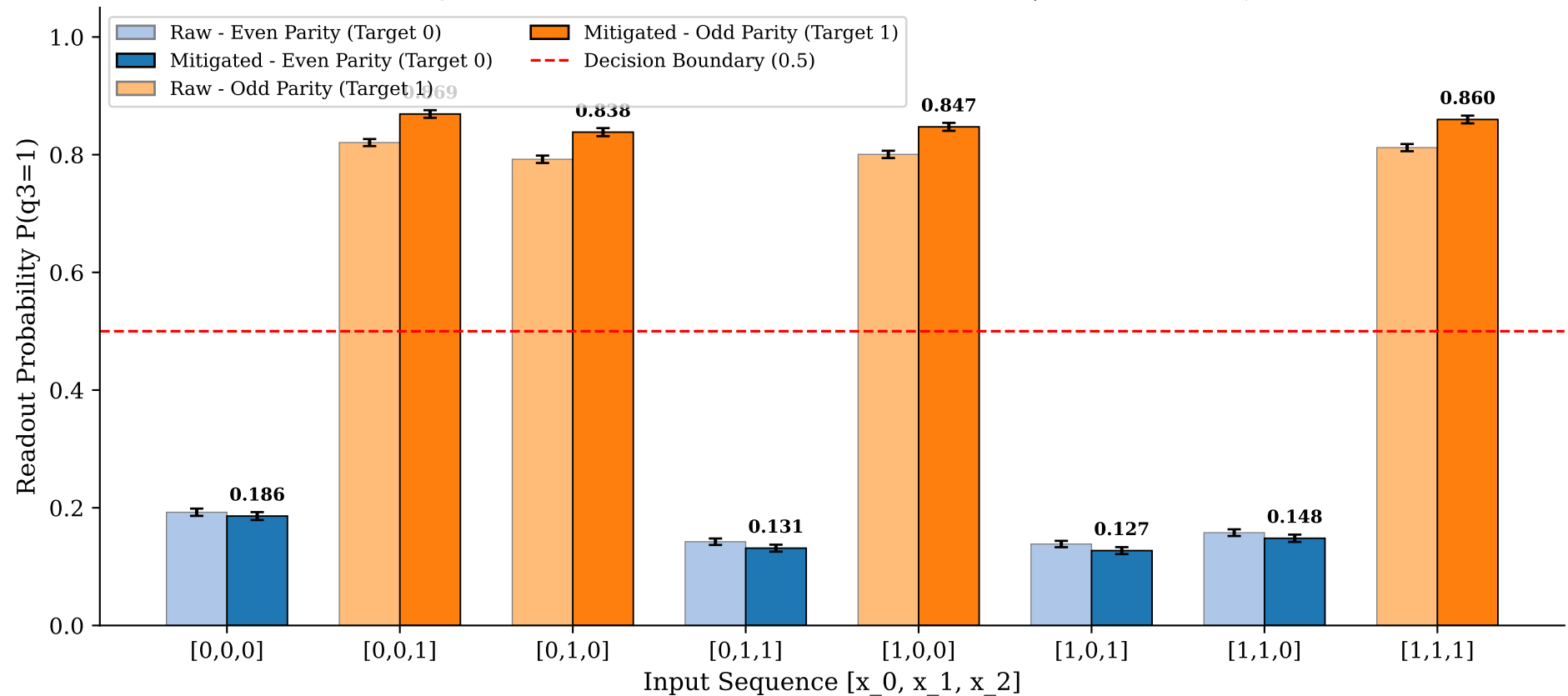
Figure 7: Physical QPU High-Shot Validation with Readout Error Mitigation (Rigetti QPU via BlueQubit, 4096 shots/circuit | 100% Accuracy)
