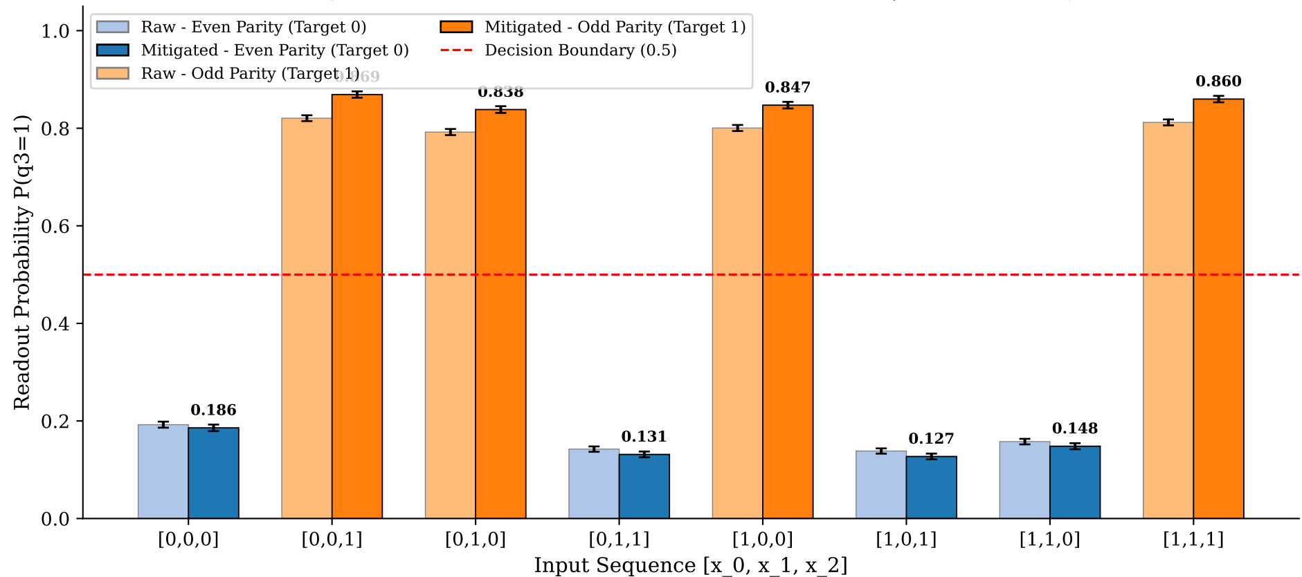
Figure 7: Physical QPU High-Shot Validation with Readout Error Mitigation (Rigetti Aspen-M-3 via BlueQubit, 4096 shots/circuit | 100% Accuracy)
