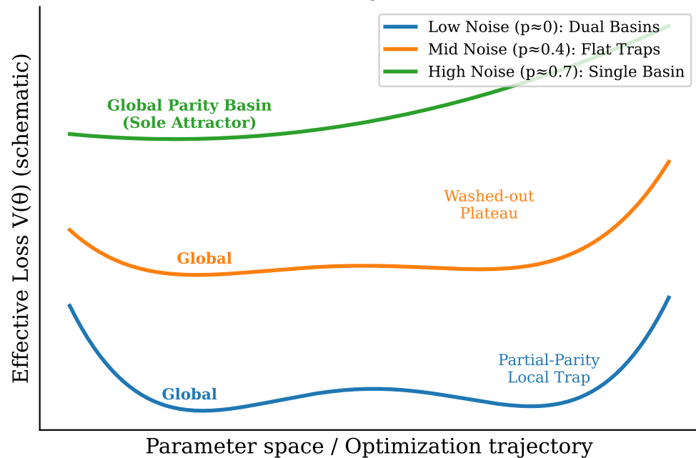
(b) Loss Landscape Regularization Schematic
