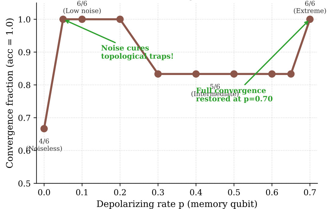
(a) Non-Monotonic Convergence vs Noise Rate p
