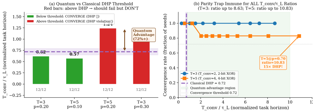
Figure 4: Quantum Parity Trap — ASYMPTOTIC IMMUNITY for Even T_{\text{conv}} Both T=3 ( \rightarrow \infty ) and T=5 ( \geq 15\times ) defeat classical DHP for all p < \text{channel capacity } p=0.75
