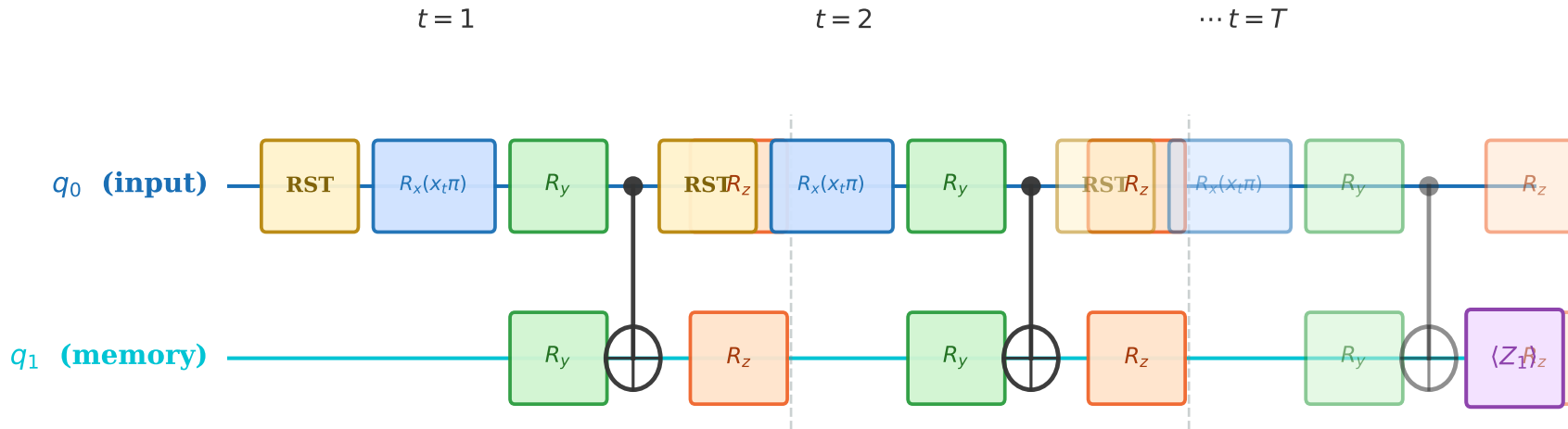
Figure 1: 2-Qubit Unitary Recurrent Quantum Circuit (URQC) Architecture
