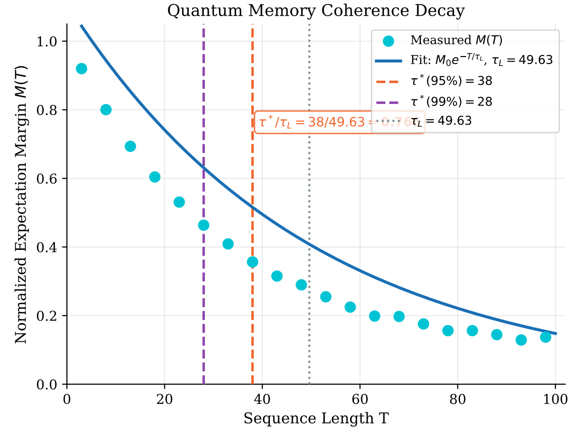
Figure 3: Aura's Continuous Coherence Decay — Fixed \theta^* Evaluated at T=3 to T=100
