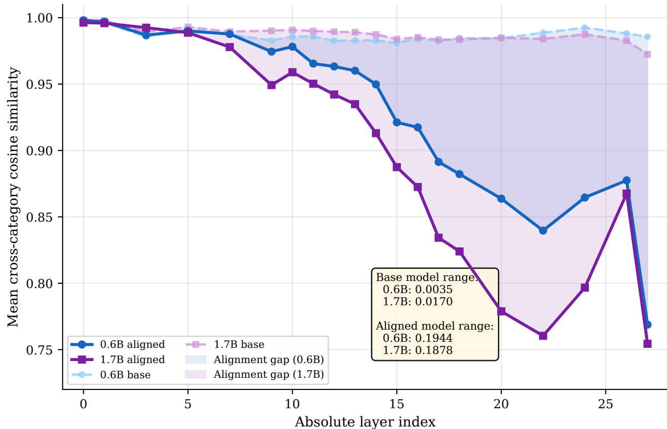
Alignment Creates Geometric Differentiation Base models nearly flat; alignment adds structure
