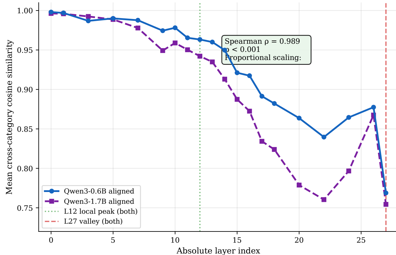
Aligned Profiles: Scale Validation Qwen3-0.6B vs 1.7B (Spearman \rho=0.989 , p<0.001 )
