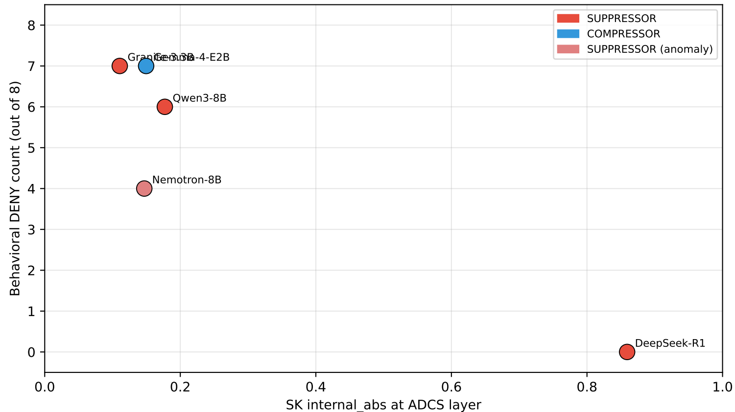
Internal Self-Knowledge Signal vs Behavioral Denial (high deny with low-moderate internal signal → suppression not integration)
