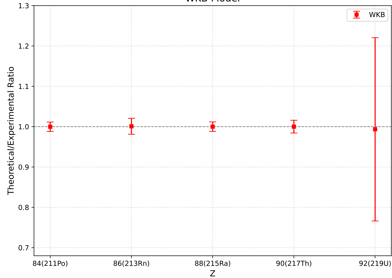
WKB Model
