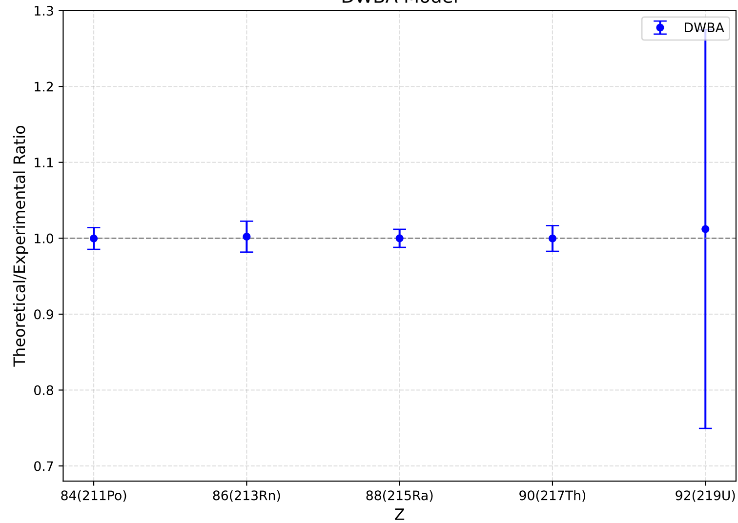
DWBA Model
