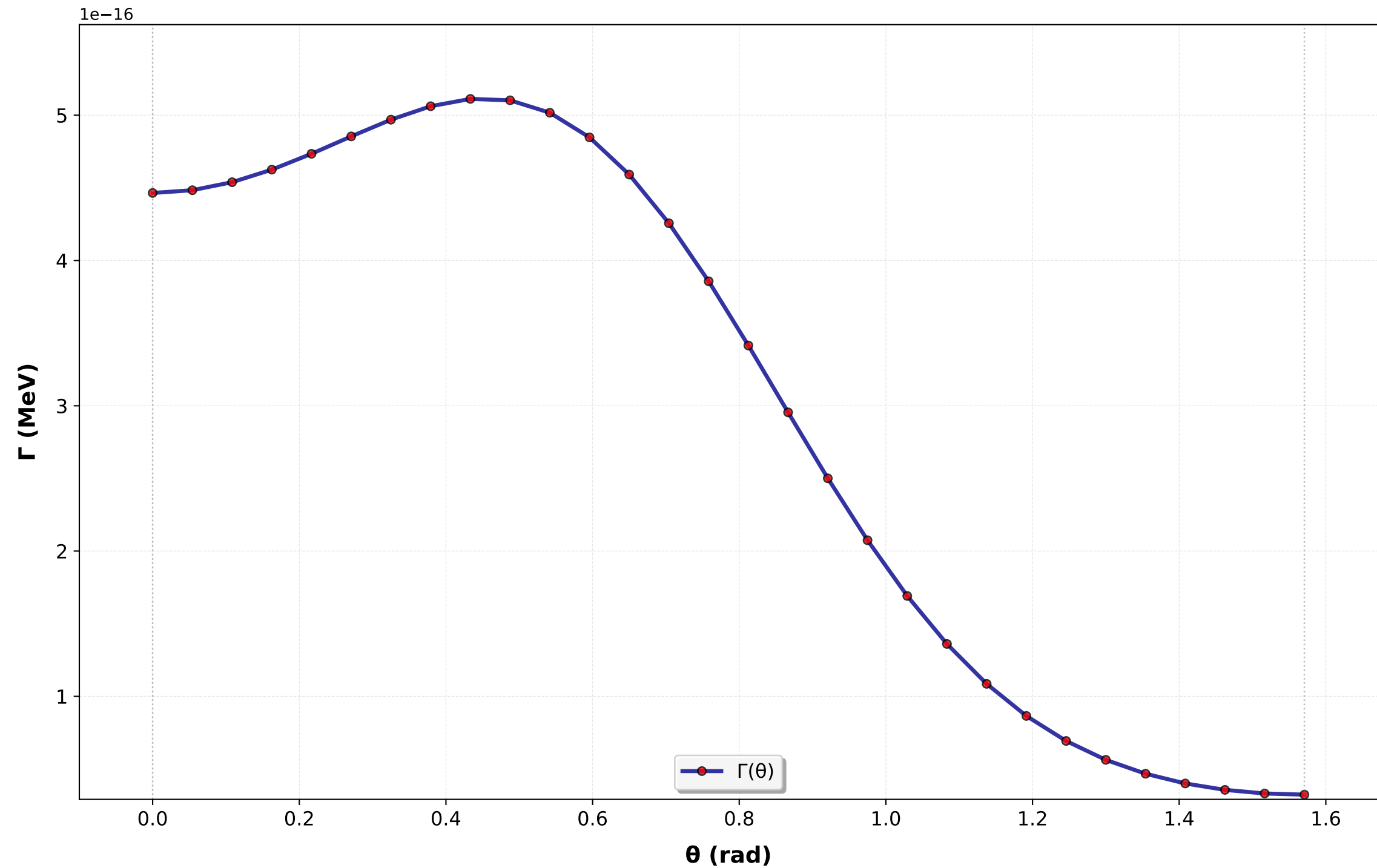
\Gamma vs \theta : Decay Width as Function of Angle
