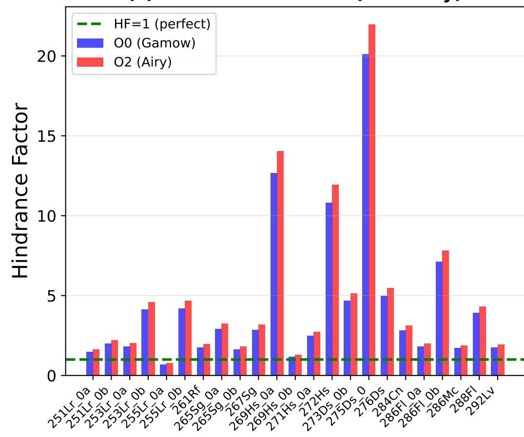
(c) Hindrance Factors ( \ell = 0 only)
