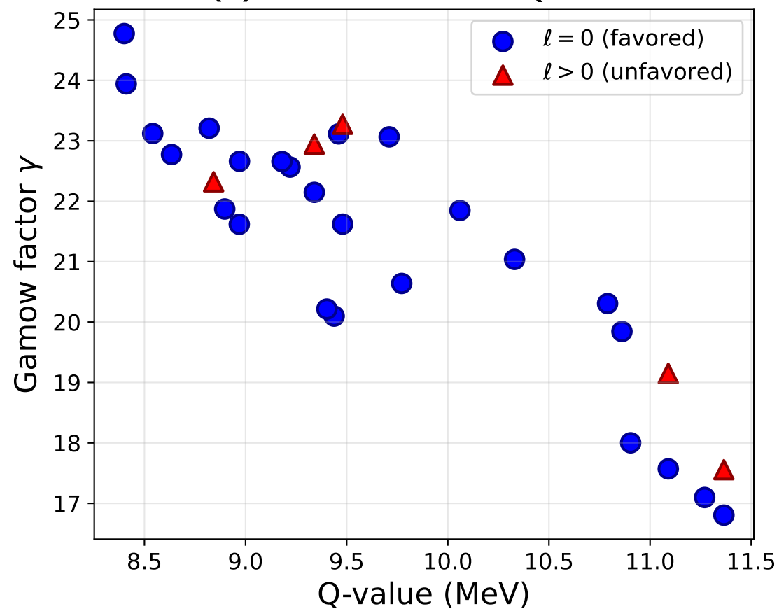
(a) Gamow Factor vs Q-value
