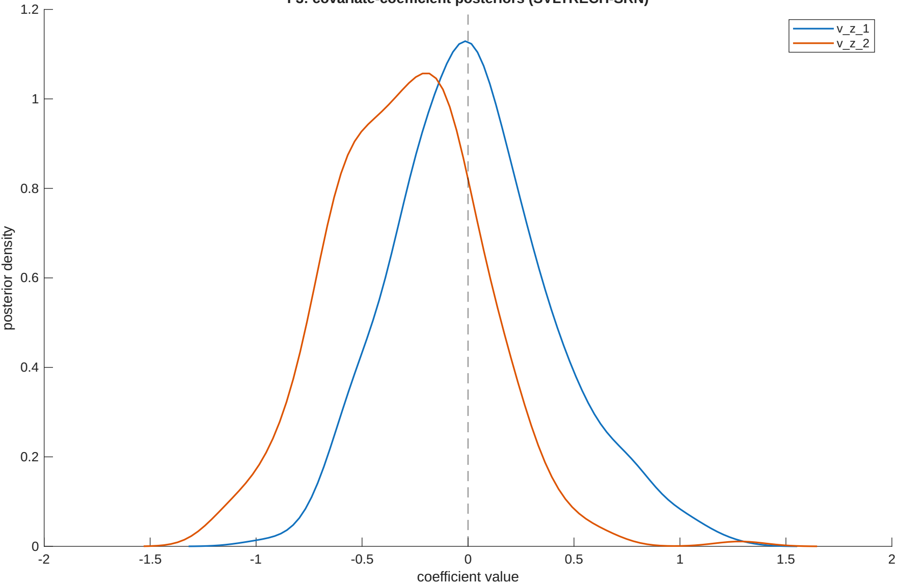
F3: covariate-coefficient posteriors (SVLTRECH-SRN)
