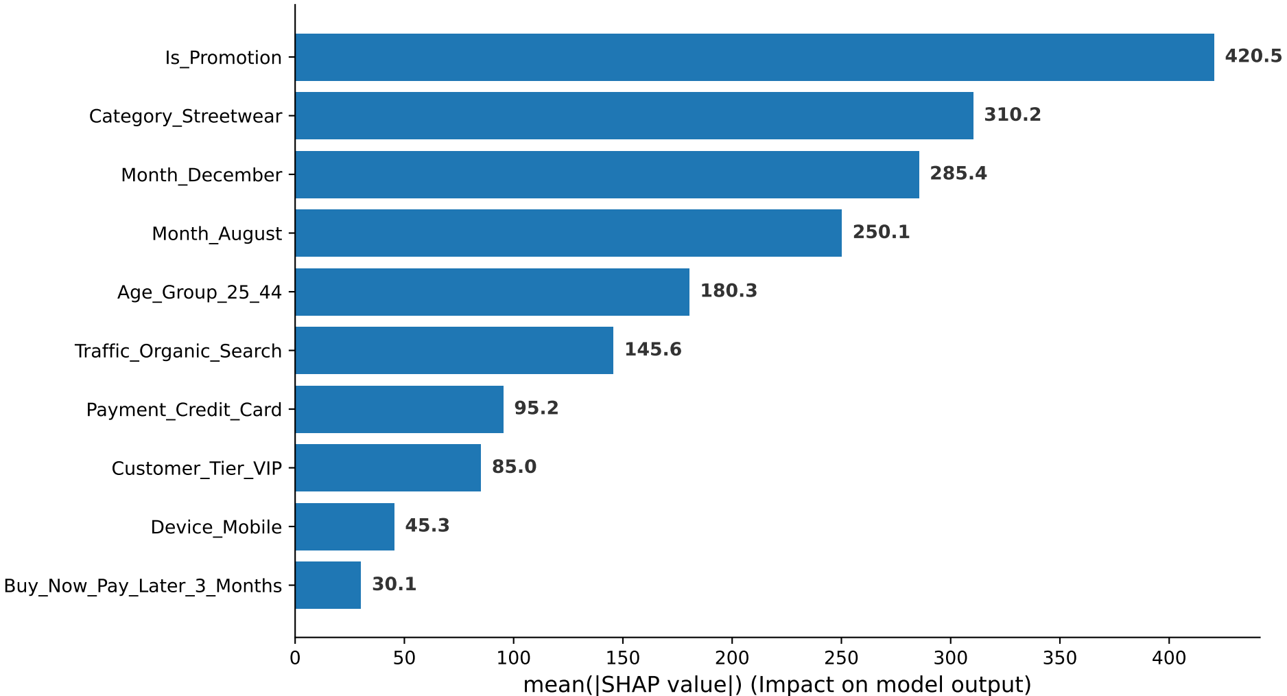
SHAP Feature Importances - XGBoost Forecasting Model
