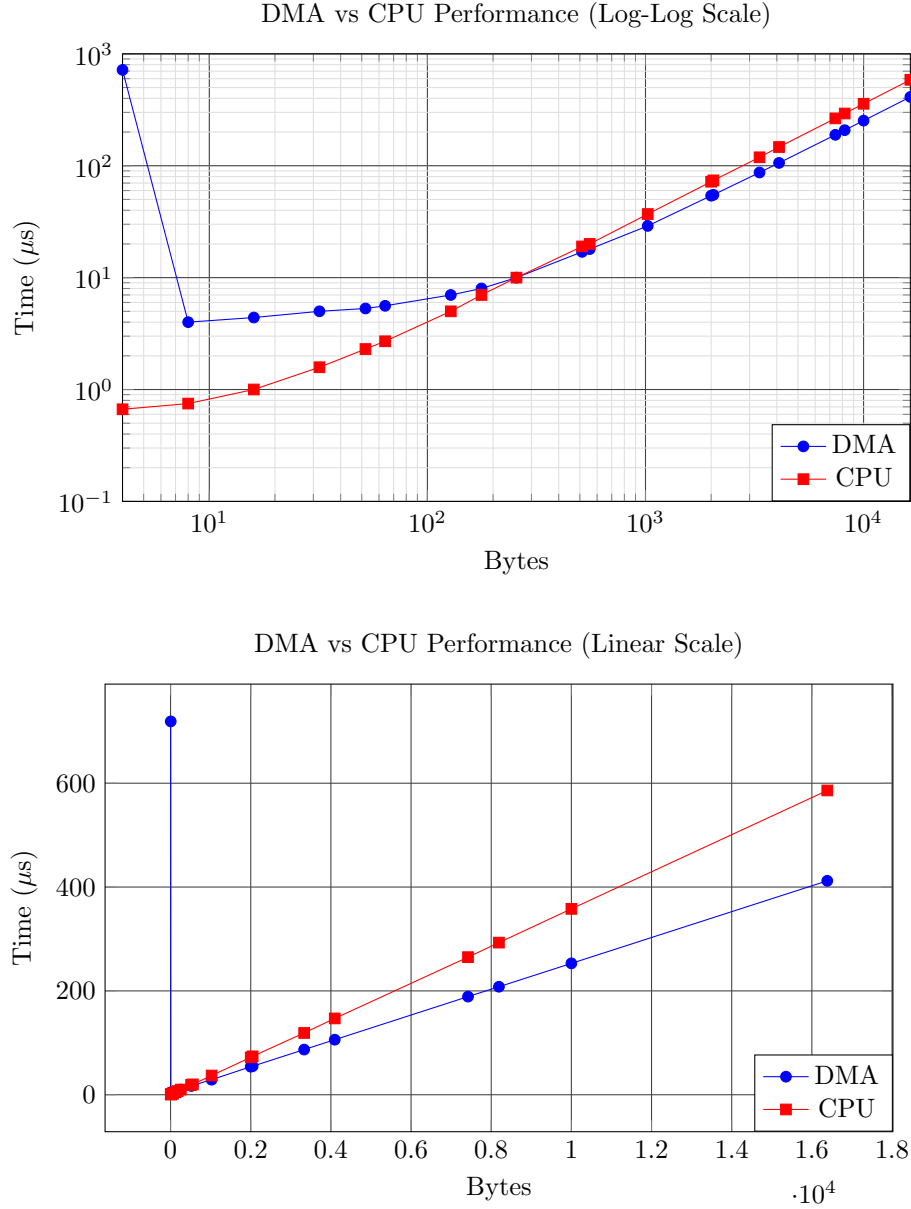
Figure 1: Comparison of DMA and CPU transfer times (in \mu s ).
