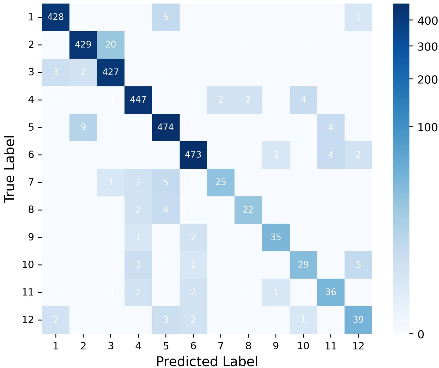
Confusion Matrix (Counts)
