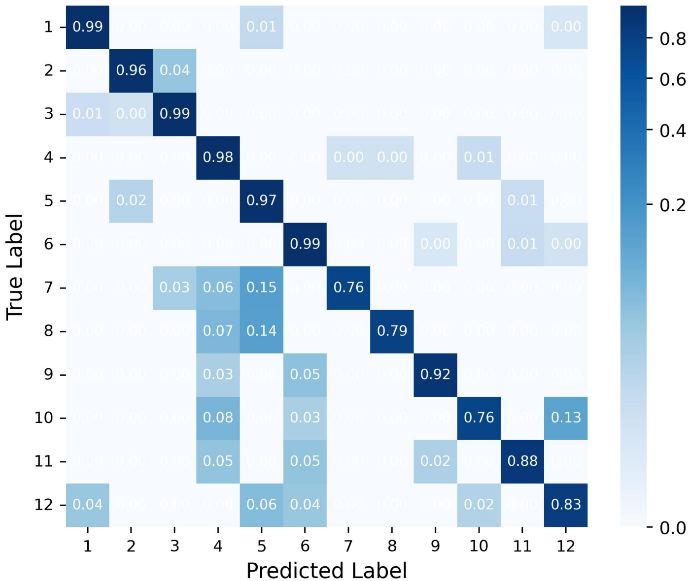
Confusion Matrix (Row-normalized)
