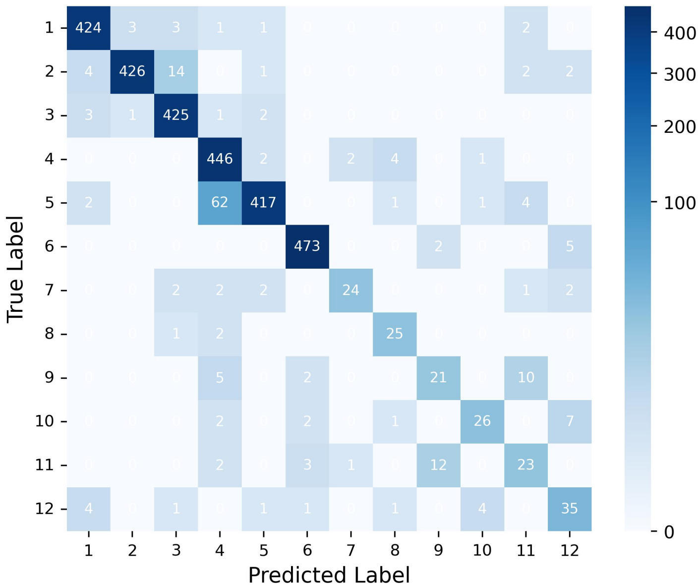
Confusion Matrix - Counts (before)
