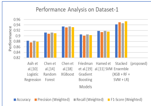
Fig. 1. Performance Analysis of Stacked Ensemble Model on Dataset-1
