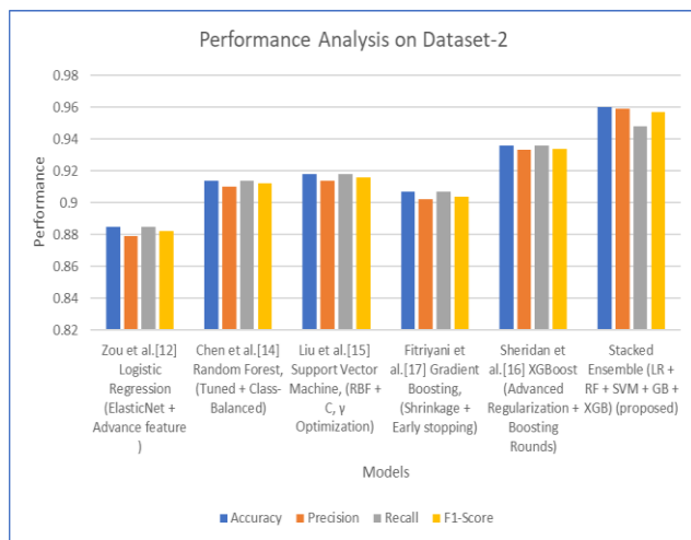
Fig. 2. Performance Analysis of Stacked Ensemble Model on Dataset-2
