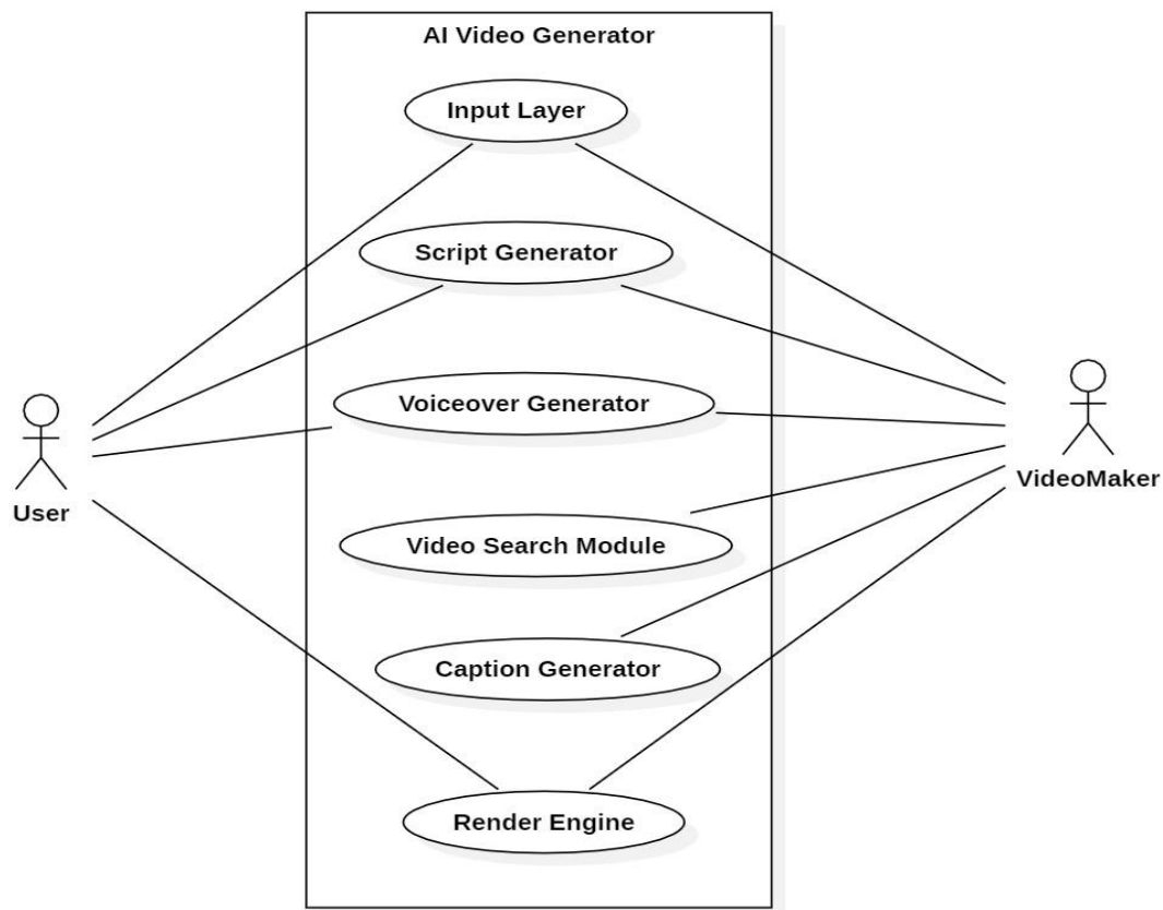
Fig 3.3 Use Case Diagram for AI-Driven Automated Video Generator for Content Creation
