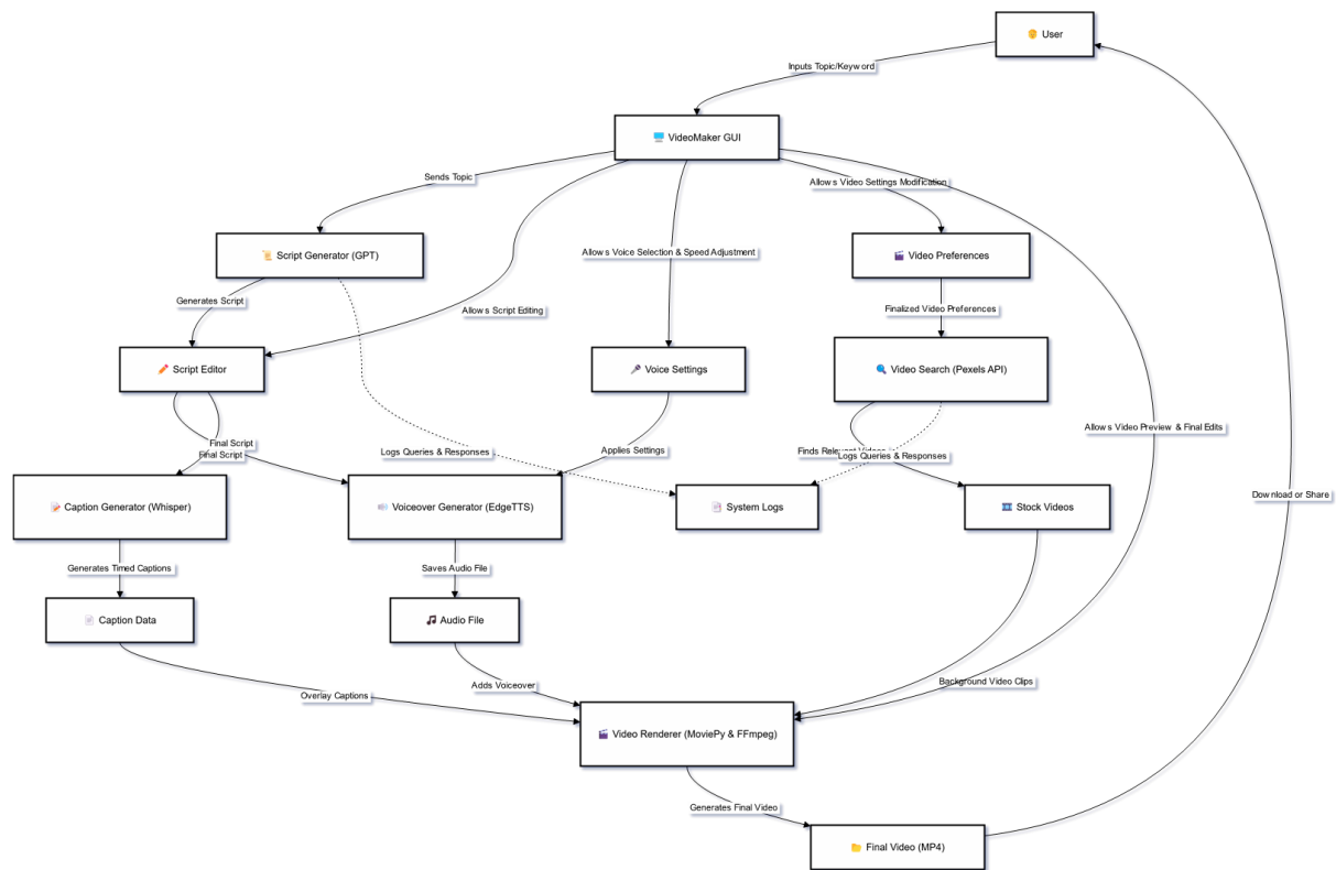
Fig 3.4 System Architecture of AI-Driven Automated Video Generator for Content Creation
