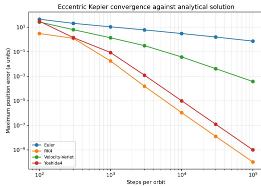
Figure 19. Eccentric-orbit global position-error convergence against the analytical Kepler solution.
