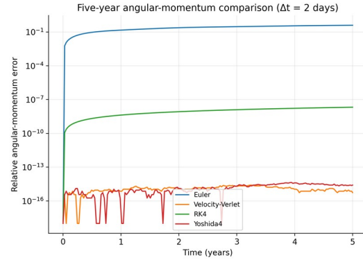
Figure 3. Relative angular-momentum error in the five-year integrator comparison.
