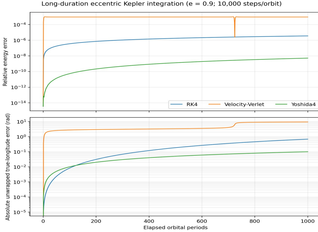
Figure 8. Once-per-orbit display of energy-error magnitude and true-longitude discrepancy for e = 0.9 over 1,000 periods at 10,000 steps/orbit. Tabulated maxima use 200 diagnostic samples per orbit.
