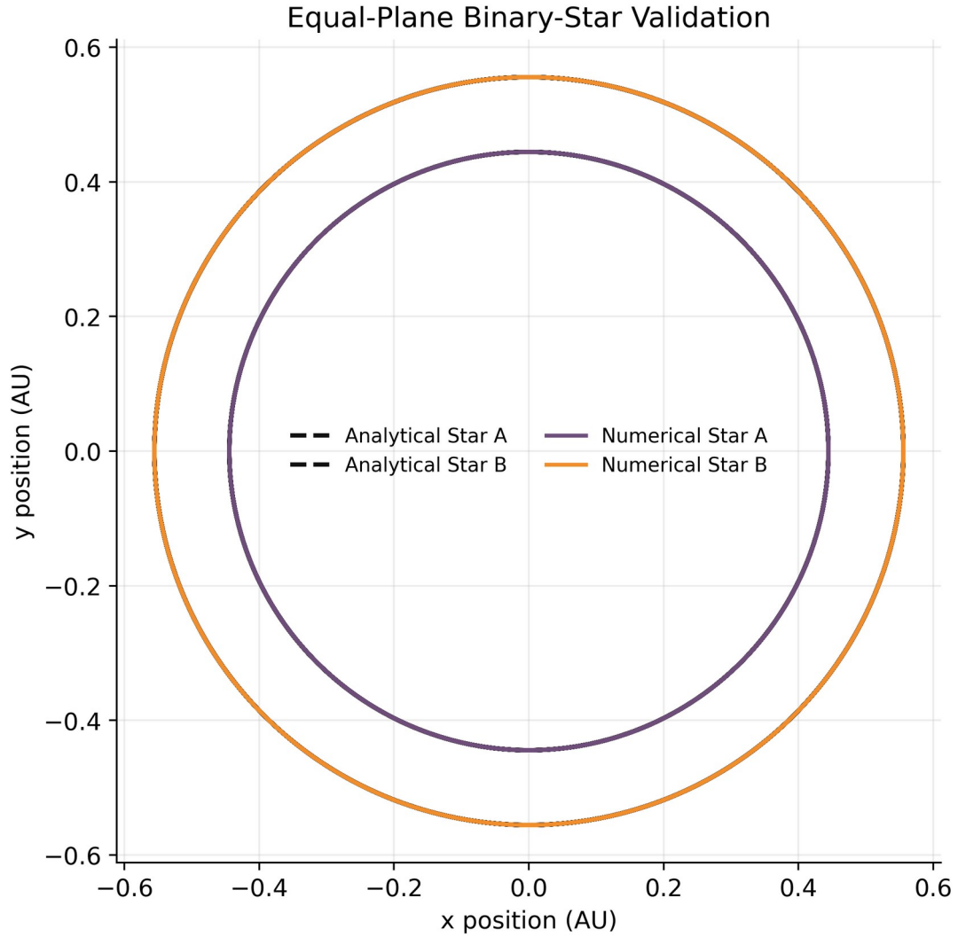
Figure 13. Numerical and analytical trajectories for the circular 1.0–0.8 solar-mass binary; axes use equal aspect ratio.
