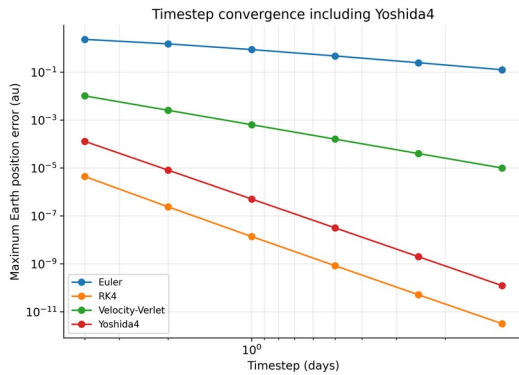
Figure 4. Maximum position error versus timestep for the main methods.
