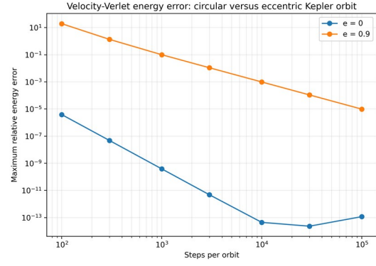
Figure 7. Velocity-Verlet energy-error slopes for circular and eccentric Kepler orbits.
