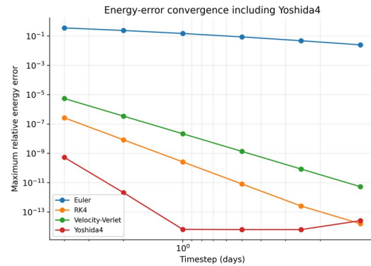
Figure 5. Maximum relative energy error versus timestep; the measured slope depends on quantity and orbit.
