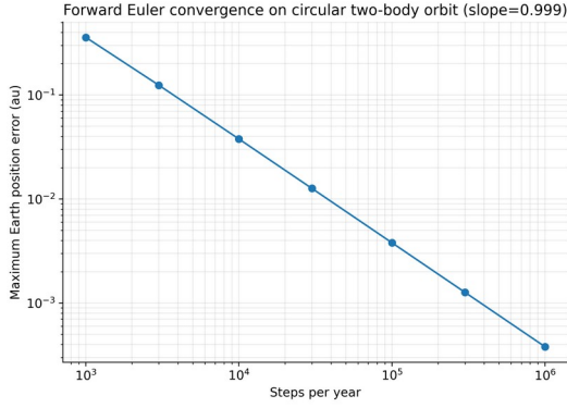
Figure 6. Fine-grid Euler convergence recovers the expected first-order trend.
