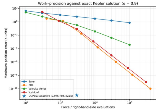
Figure 18. Work-precision comparison against the analytical eccentric Kepler solution; fixed-step work uses cached acceleration evaluation counts, while DOP853 uses the solver-reported evaluation count.
