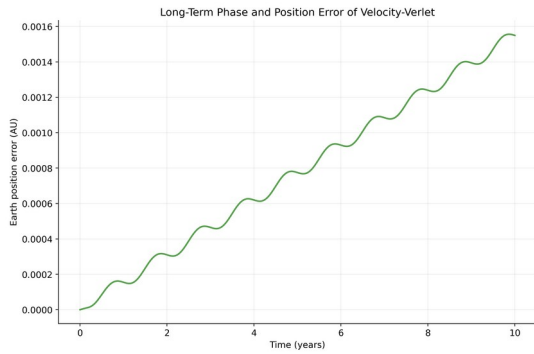
Figure 9. Position error relative to the analytical circular reference over ten years.
