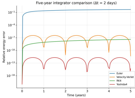
Figure 2. Relative energy error in the multi-year integrator comparison.
