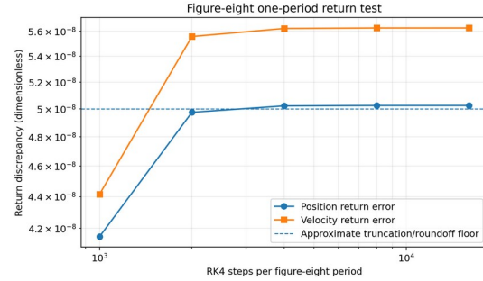
Figure 20. Figure-eight one-period return discrepancy for RK4. The plateau reflects rounded initial conditions and period, limiting its use as a convergence reference.
