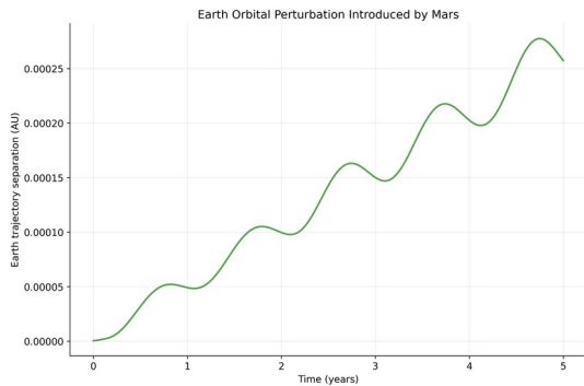
Figure 11. Earth trajectory separation with and without Mars over five years.
