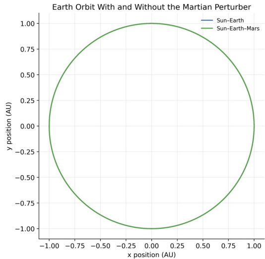
Figure 12. Two-body and three-body Earth trajectories, with equal aspect ratio.
