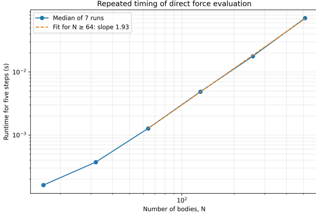
Figure 16. Repeated timing of five direct-force integration steps; points summarize repeated measurements and the fit uses the stated large- N subset.
