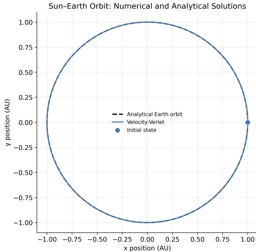
Figure 1. Numerical Sun–Earth orbit compared with the analytical circular two-body solution; spatial axes use equal scaling.
