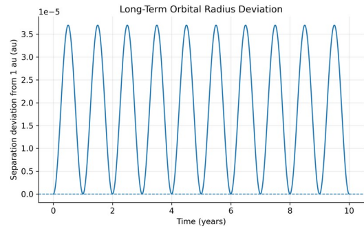
Figure 10. Earth–Sun separation over ten years; bounded radius is not exact phase agreement.
