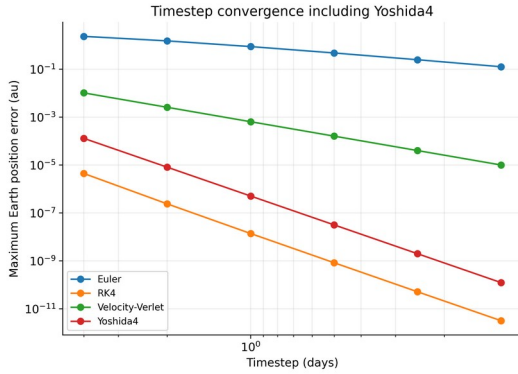
Figure 4. Maximum position error versus timestep for the main methods.
