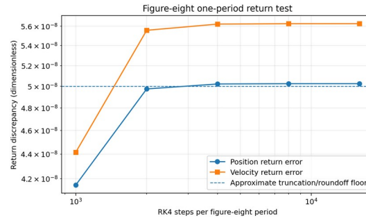
Figure 20. Figure-eight one-period return discrepancy for RK4. The plateau reflects rounded initial conditions and period, limiting its use as a convergence reference.
