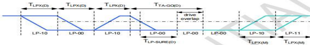
Bus turnaround (BAT) from display module to MPU timing
