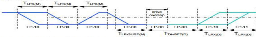
Bus turnaround (BAT) from MPU to display module timing
