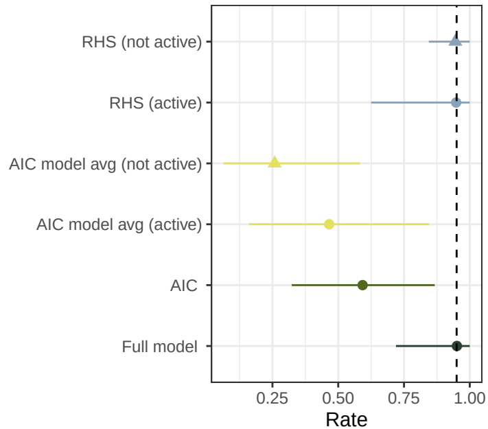
CI coverage
