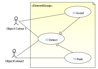
Fig. 3. Use Case Diagram(Object-Oriented)
