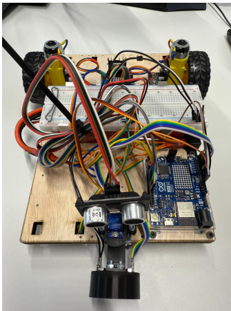
Fig. 8. Robot Assembly
