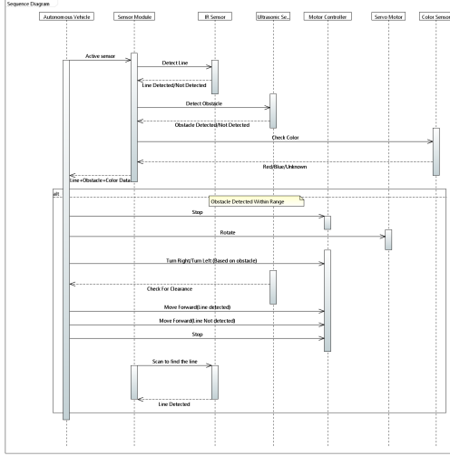
Fig. 16. SequenceDiagram (full page view in Appendix B)
