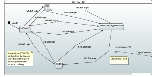
Fig. 14. FollowLineStateMachine
