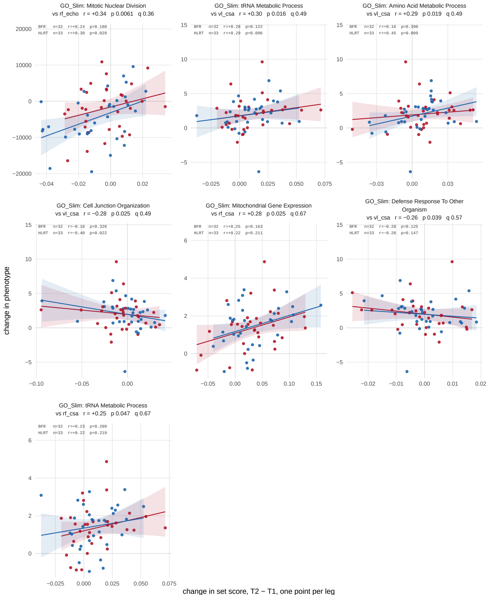
S16 Figure. Training response against phenotype, all legs, GO_Slim. All 7 GO_Slim set-outcome pairs whose Spearman correlation reaches nominal p in the pooled analysis (65 legs, both arms pooled), smallest p first. Lines are fitted within each arm; the header r is the pooled correlation and the inset gives it within each arm. q from BH within collection and outcome. Nominal p , uncorrected: chance alone returns 3.0 of the 59 GO_Slim sets. Data: set_association and set_by_arm sheets of 05_classify_and_associate_sets.xlsx.
