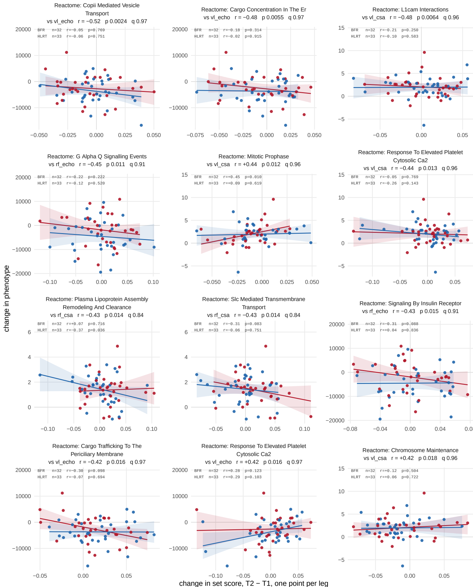
S17 Figure (page 1 of 4). BFR minus HLRT, within participant, Reactome. All 44 Reactome set-outcome pairs whose Spearman correlation reaches nominal p in the differential analysis (32 paired participants), smallest p first. Lines are fitted within each arm; the header r is the differential correlation and the inset gives it within each arm. q from BH within collection and outcome. Nominal p, uncorrected: chance alone returns 21.5 of the 430 Reactome sets. Data: set_association and set_by_arm sheets of 05_classify_and_associate_sets.xlsx.
