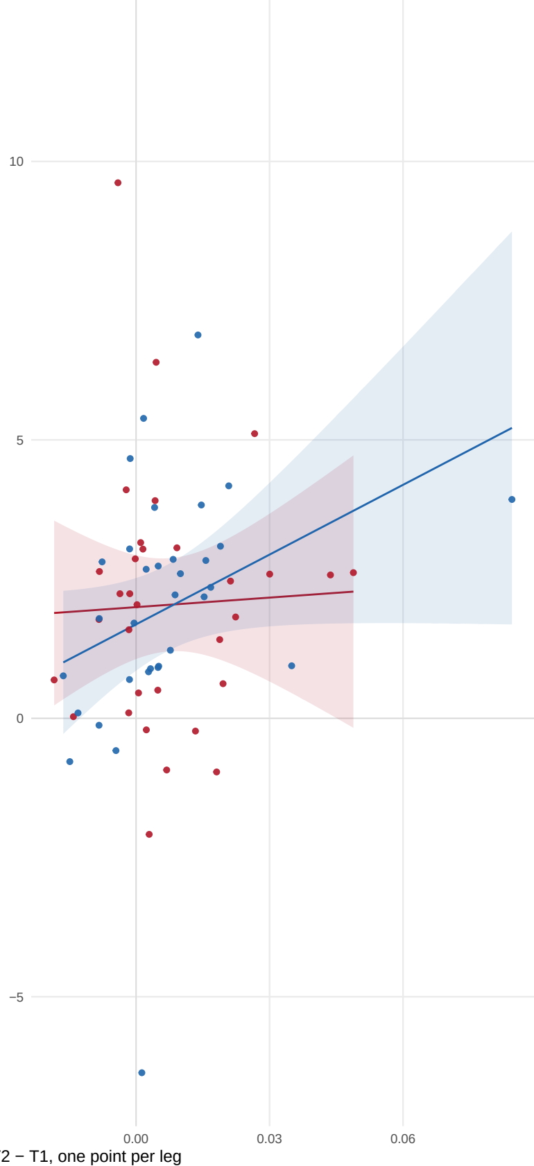
S16 Figure (page 4 of 4). Training response against phenotype, all legs, Reactome. All 38 Reactome set-outcome pairs whose Spearman correlation reaches nominal p in the pooled analysis (65 legs, both arms pooled), smallest p first. Lines are fitted within each arm; the header r is the pooled correlation and the inset gives it within each arm. q from BH within collection and outcome. Nominal p , uncorrected: chance alone returns 21.5 of the 430 Reactome sets. Data: set_association and set_by_arm sheets of 05_classify_and_associate_sets.xlsx.
