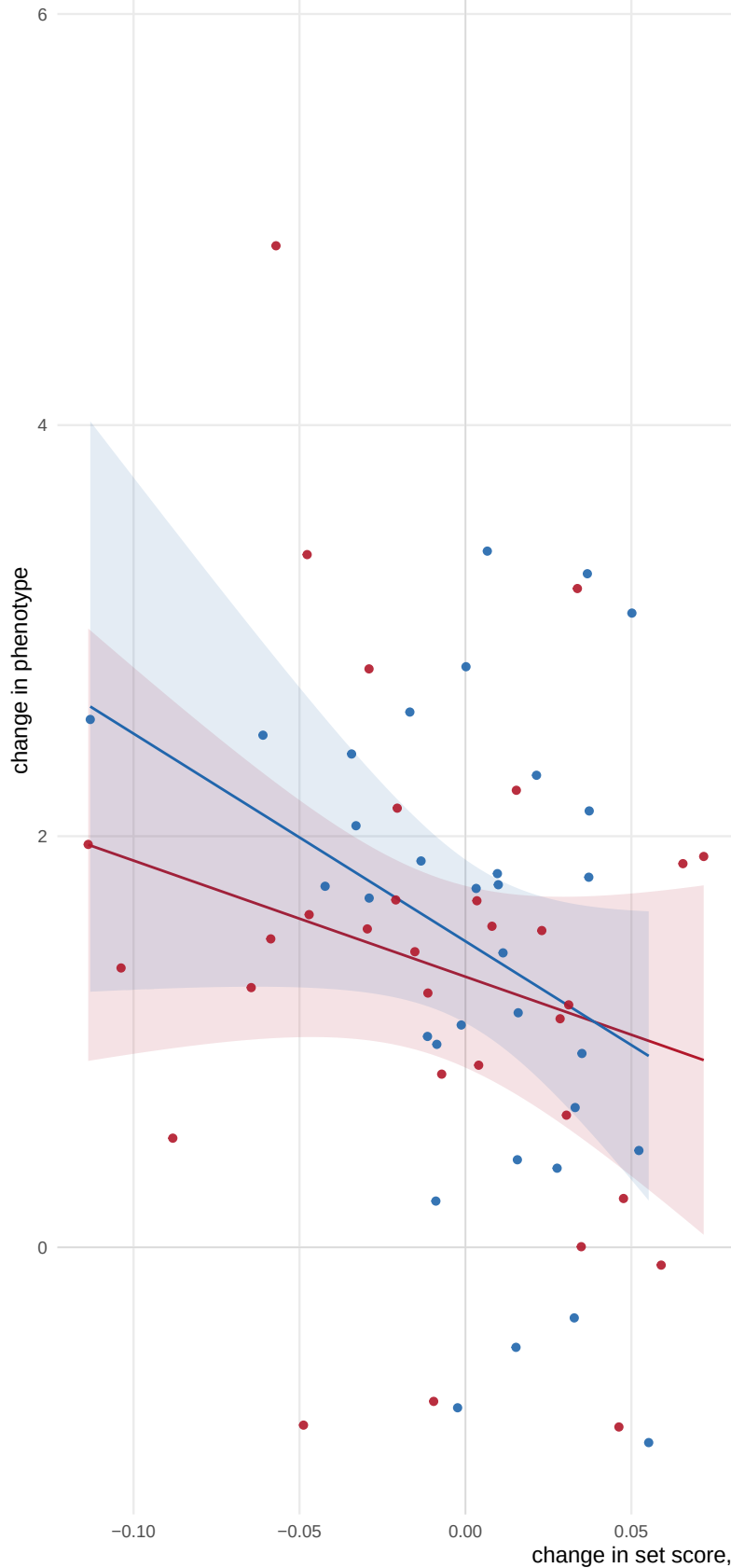
S16 Figure (page 4 of 4). Training response against phenotype, all legs, Reactome. All 38 Reactome set-outcome pairs whose Spearman correlation reaches nominal p in the pooled analysis (65 legs, both arms pooled), smallest p first. Lines are fitted within each arm; the header r is the pooled correlation and the inset gives it within each arm. q from BH within collection and outcome. Nominal p , uncorrected: chance alone returns 21.5 of the 430 Reactome sets. Data: set_association and set_by_arm sheets of 05_classify_and_associate_sets.xlsx.
