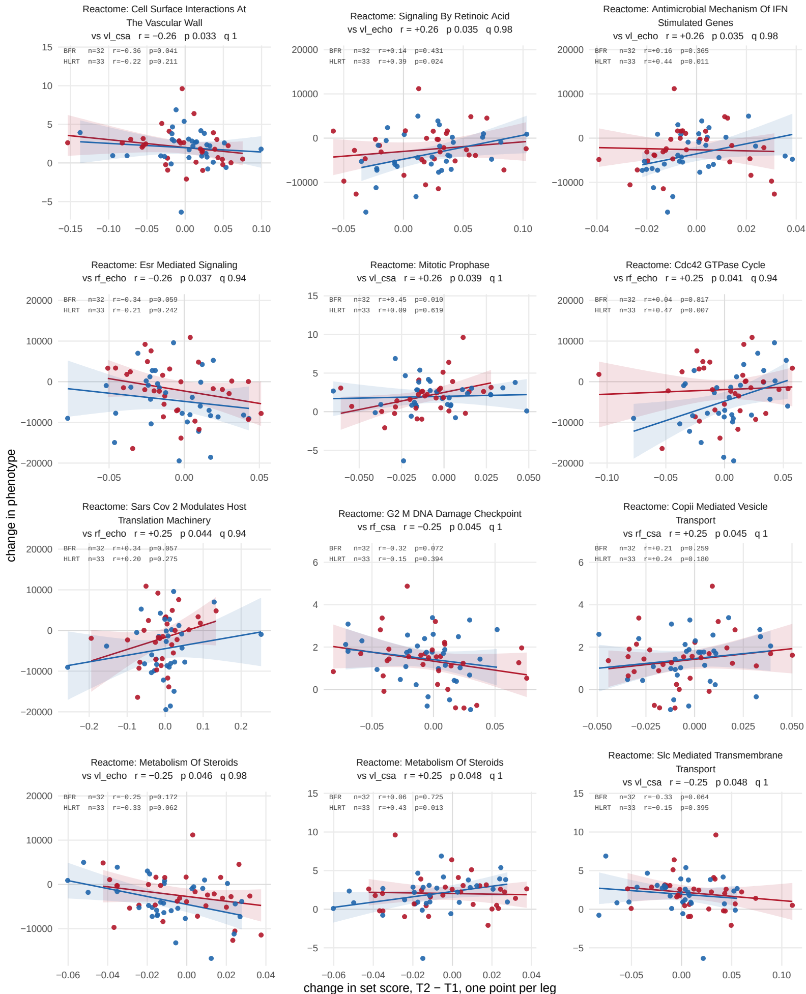
S16 Figure (page 3 of 4). Training response against phenotype, all legs, Reactome. All 38 Reactome set-outcome pairs whose Spearman correlation reaches nominal p in the pooled analysis (65 legs, both arms pooled), smallest p first. Lines are fitted within each arm; the header r is the pooled correlation and the inset gives it within each arm. q from BH within collection and outcome. Nominal p , uncorrected: chance alone returns 21.5 of the 430 Reactome sets. Data: set_association and set_by_arm sheets of 05_classify_and_associate_sets.xlsx.
