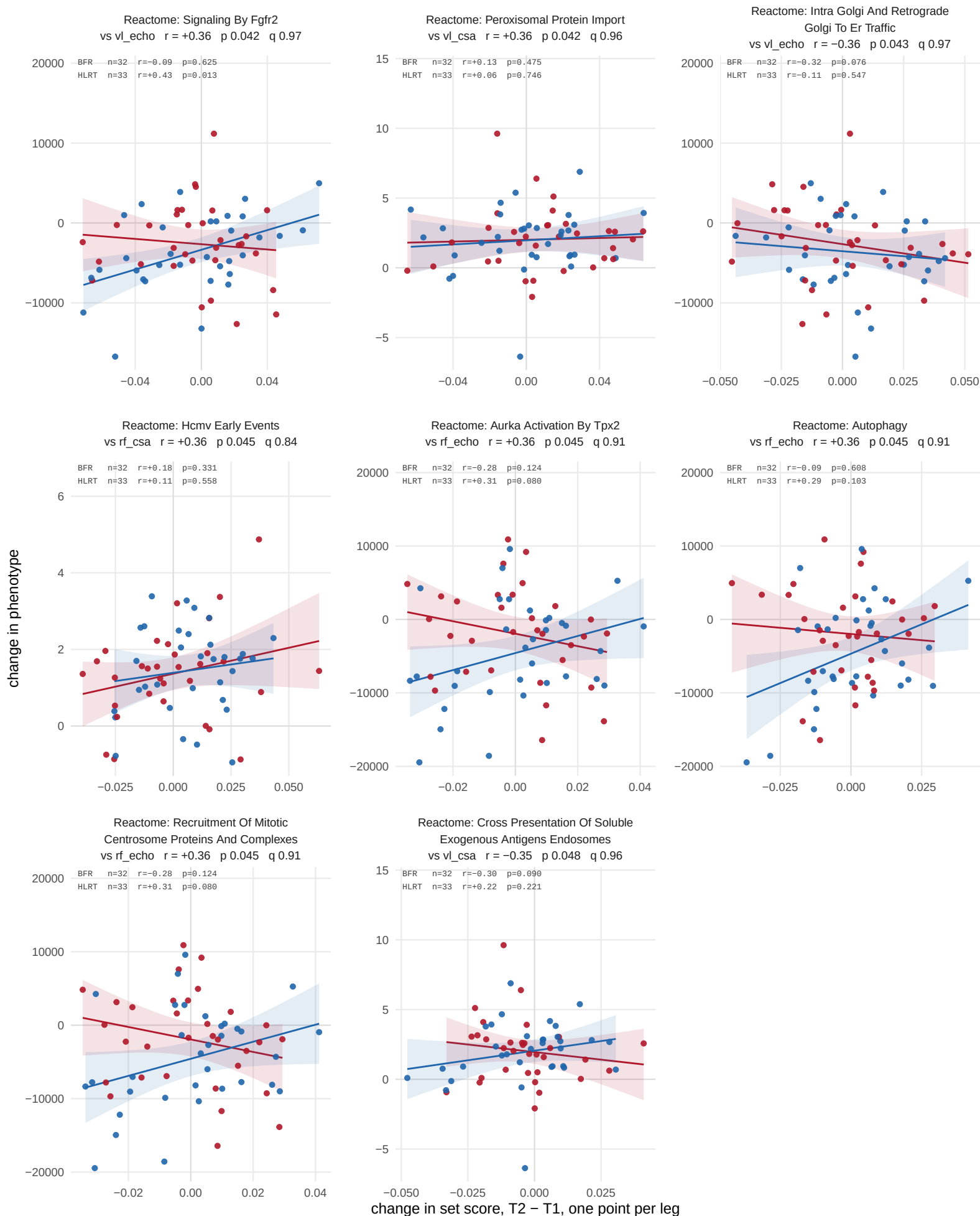
S17 Figure (page 4 of 4). BFR minus HLRT, within participant, Reactome. All 44 Reactome set-outcome pairs whose Spearman correlation reaches nominal p in the differential analysis (32 paired participants), smallest p first. Lines are fitted within each arm; the header r is the differential correlation and the inset gives it within each arm. q from BH within collection and outcome. Nominal p , uncorrected: chance alone returns 21.5 of the 430 Reactome sets. Data: set_association and set_by_arm sheets of 05_classify_and_associate_sets.xlsx.
