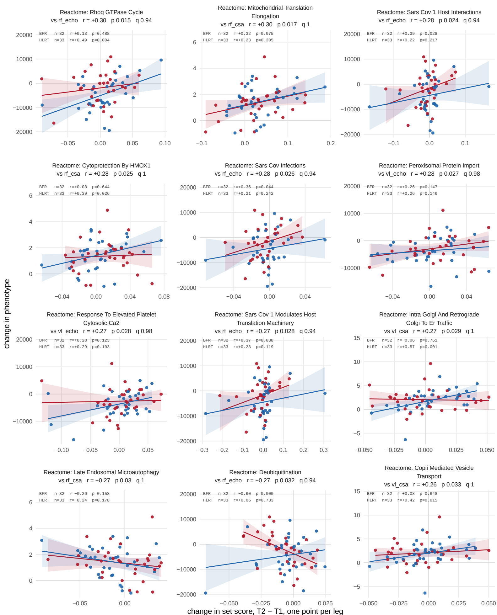
S16 Figure (page 2 of 4). Training response against phenotype, all legs, Reactome. All 38 Reactome set-outcome pairs whose Spearman correlation reaches nominal p in the pooled analysis (65 legs, both arms pooled), smallest p first. Lines are fitted within each arm; the header r is the pooled correlation and the inset gives it within each arm. q from BH within collection and outcome. Nominal p , uncorrected: chance alone returns 21.5 of the 430 Reactome sets. Data: set_association and set_by_arm sheets of 05_classify_and_associate_sets.xlsx.
