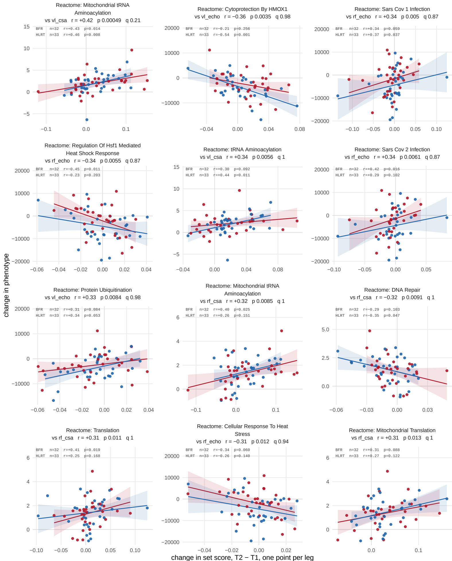
S16 Figure (page 1 of 4). Training response against phenotype, all legs, Reactome. All 38 Reactome set-outcome pairs whose Spearman correlation reaches nominal p in the pooled analysis (65 legs, both arms pooled), smallest p first. Lines are fitted within each arm; the header r is the pooled correlation and the inset gives it within each arm. q from BH within collection and outcome. Nominal p , uncorrected: chance alone returns 21.5 of the 430 Reactome sets. Data: set_association and set_by_arm sheets of 05_classify_and_associate_sets.xlsx.
