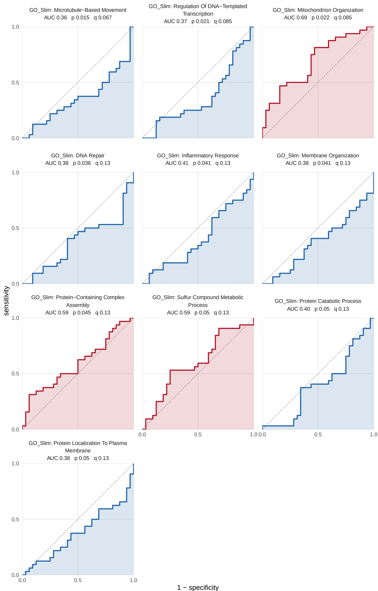
S12 Figure (page 2 of 2). Pre to post, BFR, GO_Slim. ROC curves for all 22 GO_Slim sets whose singscore separates the groups at nominal p, across 32 paired legs, smallest p first. AUC has its direction fixed: red separates higher in post, blue lower. Shading is area under the curve, dashed line chance. p from the paired Wilcoxon signed-rank test, q from BH within collection and task. Nominal p, uncorrected: chance alone returns 3.0 of the 59 GO_Slim sets. Data: set_auc sheet of 05_classify_and_associate_sets.xlsx.
