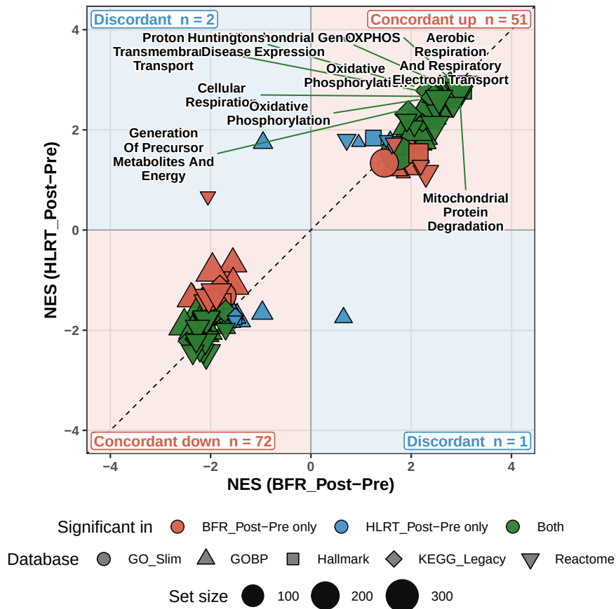
S10 Figure. NES concordance, all collections. fgsea NES for each of 1990 sets in BFR_Post-Pre (x) against HLRT_Post-Pre (y). (A) Every set. (B) Sets that survived collapsePathways in either contrast. Points are fgsea sets; grey reach neither threshold, coloured are significant (BH < 0.05 within contrast) in one or both. Shaded quadrants move the same way in both contrasts, with their counts in the corners; dashed line is identity. The subtitle gives Spearman's rho across the plotted sets. Data: nes_scatter sheet of 03_enrich_scatter_fgsea.xlsx.
