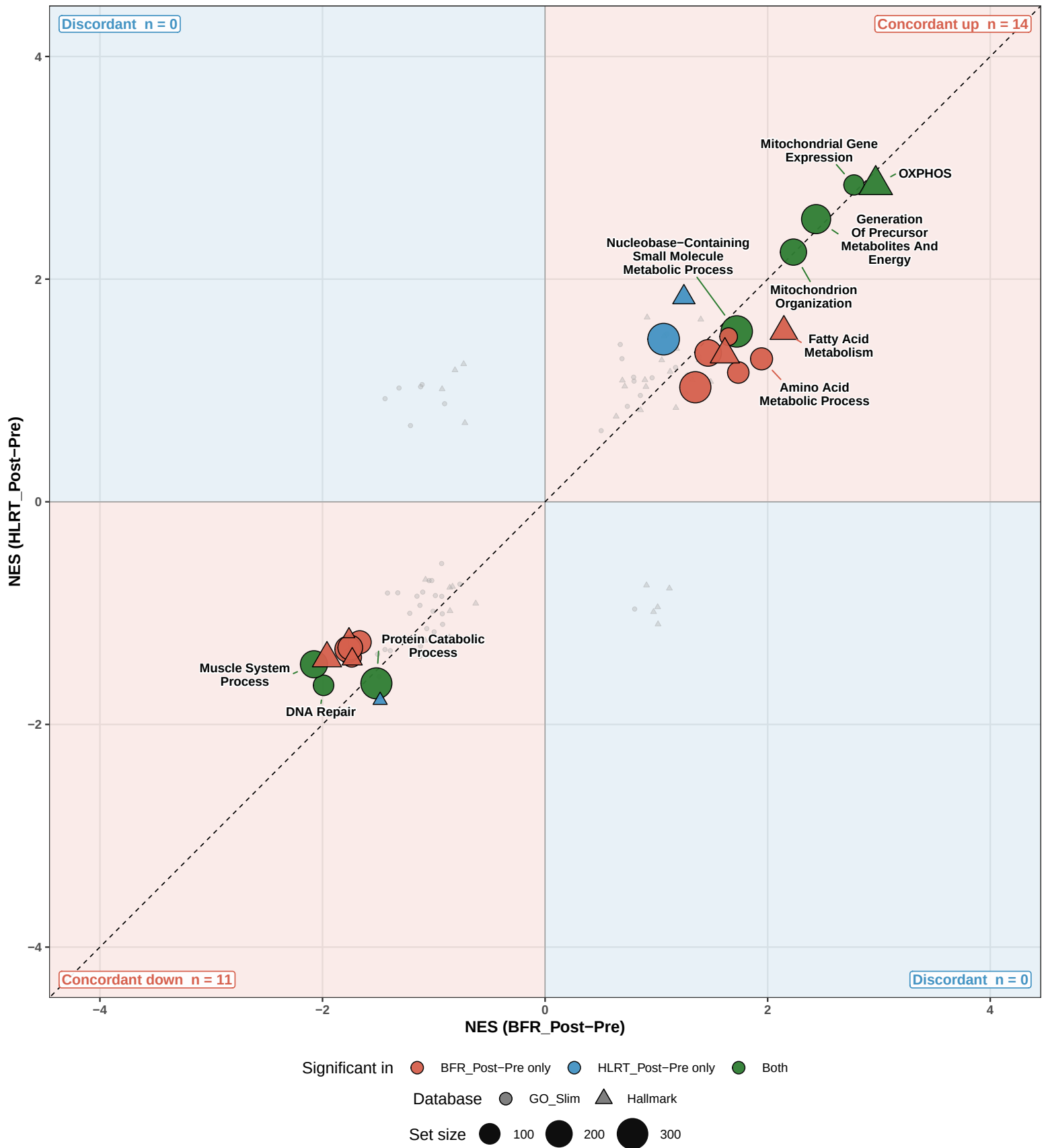
S11 Figure. NES concordance, Hallmark and GO Slim. All 100 Hallmark and GO Slim sets, whose members do not nest. Points are fgsea sets; grey reach neither threshold, coloured are significant (BH < 0.05 within contrast) in one or both. Shaded quadrants move the same way in both contrasts, with their counts in the corners; dashed line is identity. The subtitle gives Spearman's rho across the plotted sets. Data: nes_scatter sheet of 03_enrich_scatter_fgsea.xlsx.
