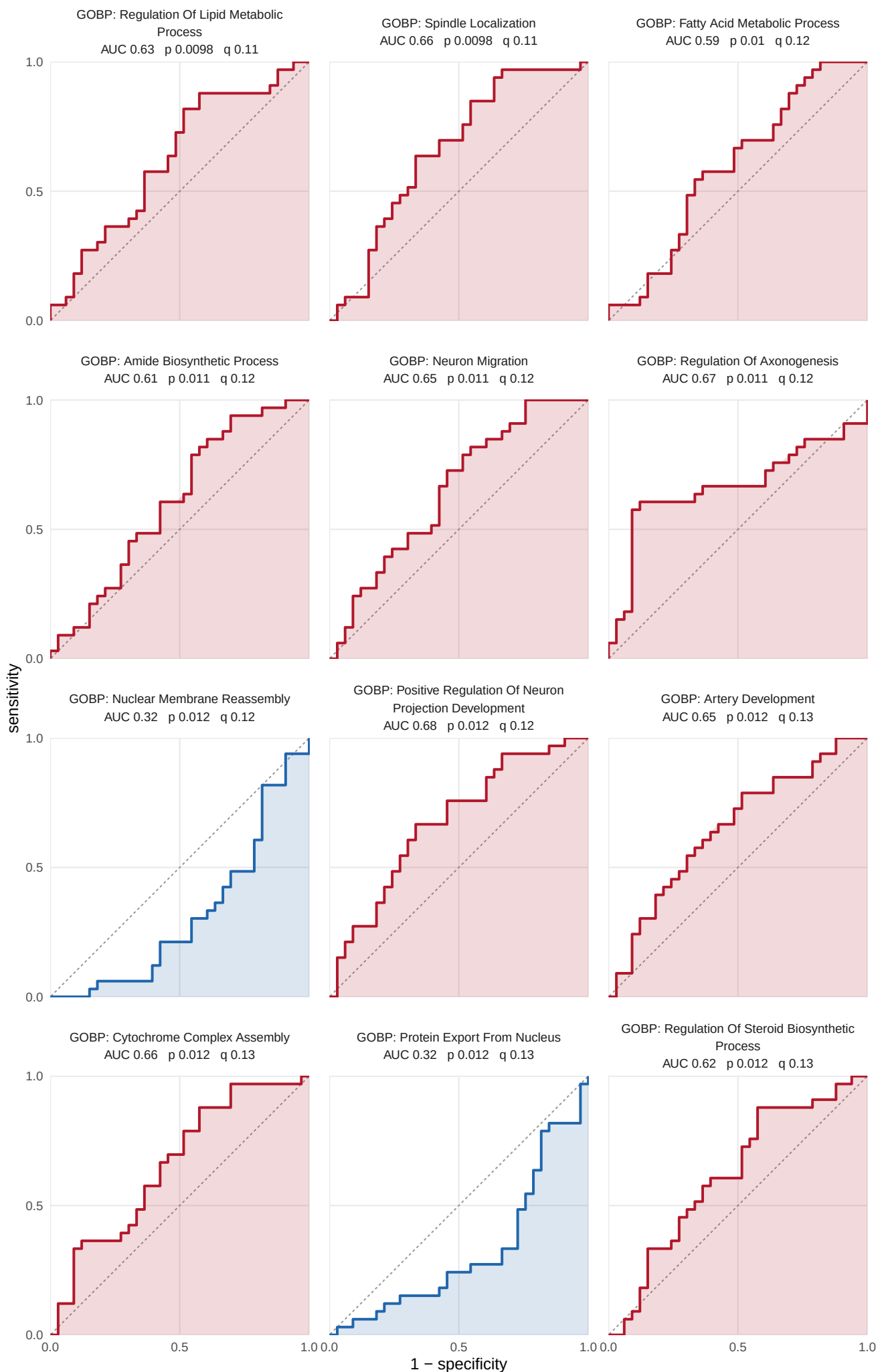
S13 Figure (page 11 of 22). Pre to post, HLRT, GOBP. ROC curves for all 255 GOBP sets whose singscore separates the groups at nominal p, across 33 paired legs, smallest p first. AUC has its direction fixed: red separates higher in post, blue lower. Shading is area under the curve, dashed line chance. p from the paired Wilcoxon signed-rank test, q from BH within collection and task. Nominal p, uncorrected: chance alone returns 68.3 of the 1366 GOBP sets. Data: set_auc sheet of 05_set_classification.xlsx.
