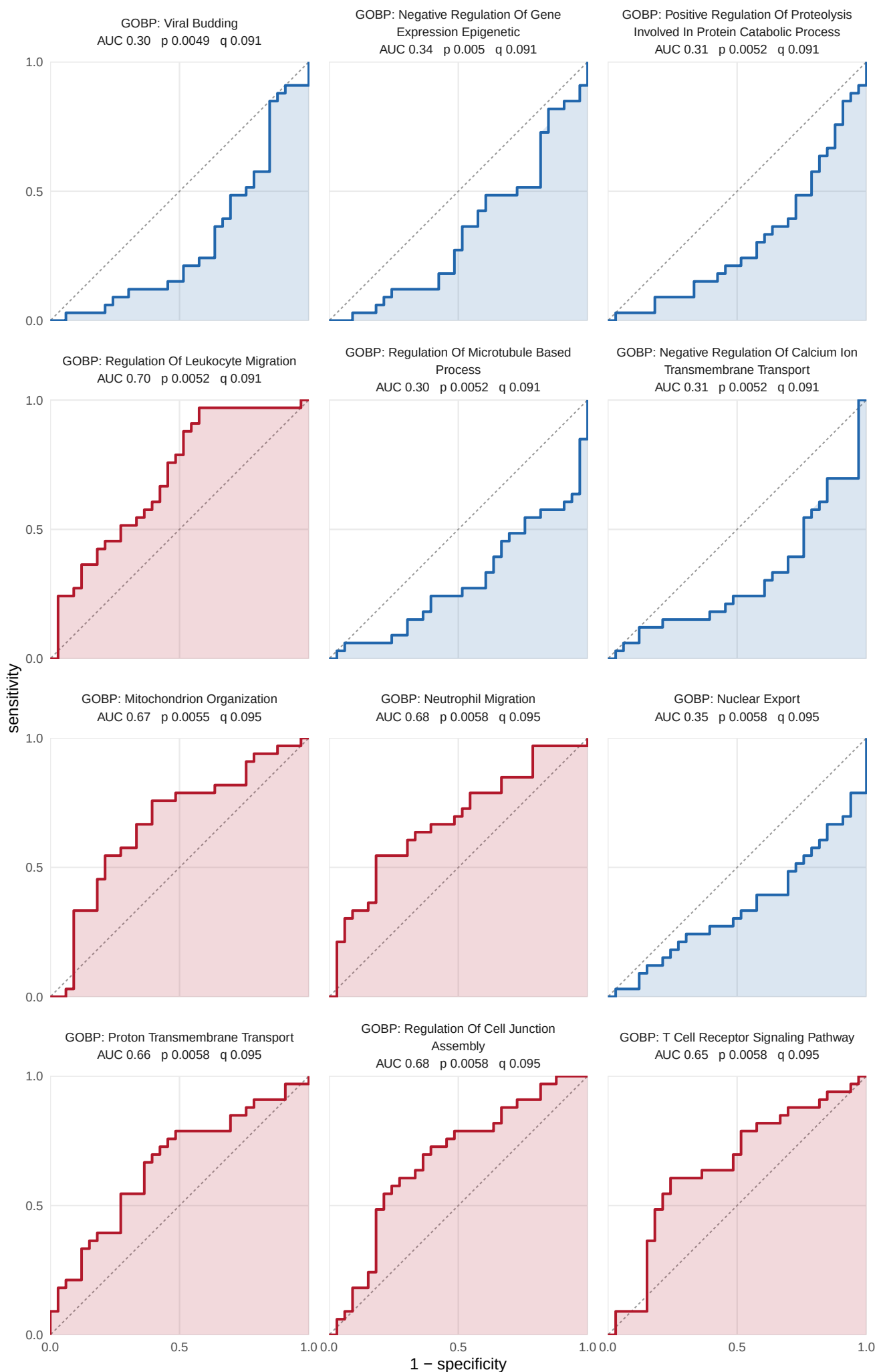
S13 Figure (page 7 of 22). Pre to post, HLRT, GOBP. ROC curves for all 255 GOBP sets whose singscore separates the groups at nominal p, across 33 paired legs, smallest p first. AUC has its direction fixed: red separates higher in post, blue lower. Shading is area under the curve, dashed line chance. p from the paired Wilcoxon signed-rank test, q from BH within collection and task. Nominal p, uncorrected: chance alone returns 68.3 of the 1366 GOBP sets. Data: set_auc sheet of 05_set_classification.xlsx.
