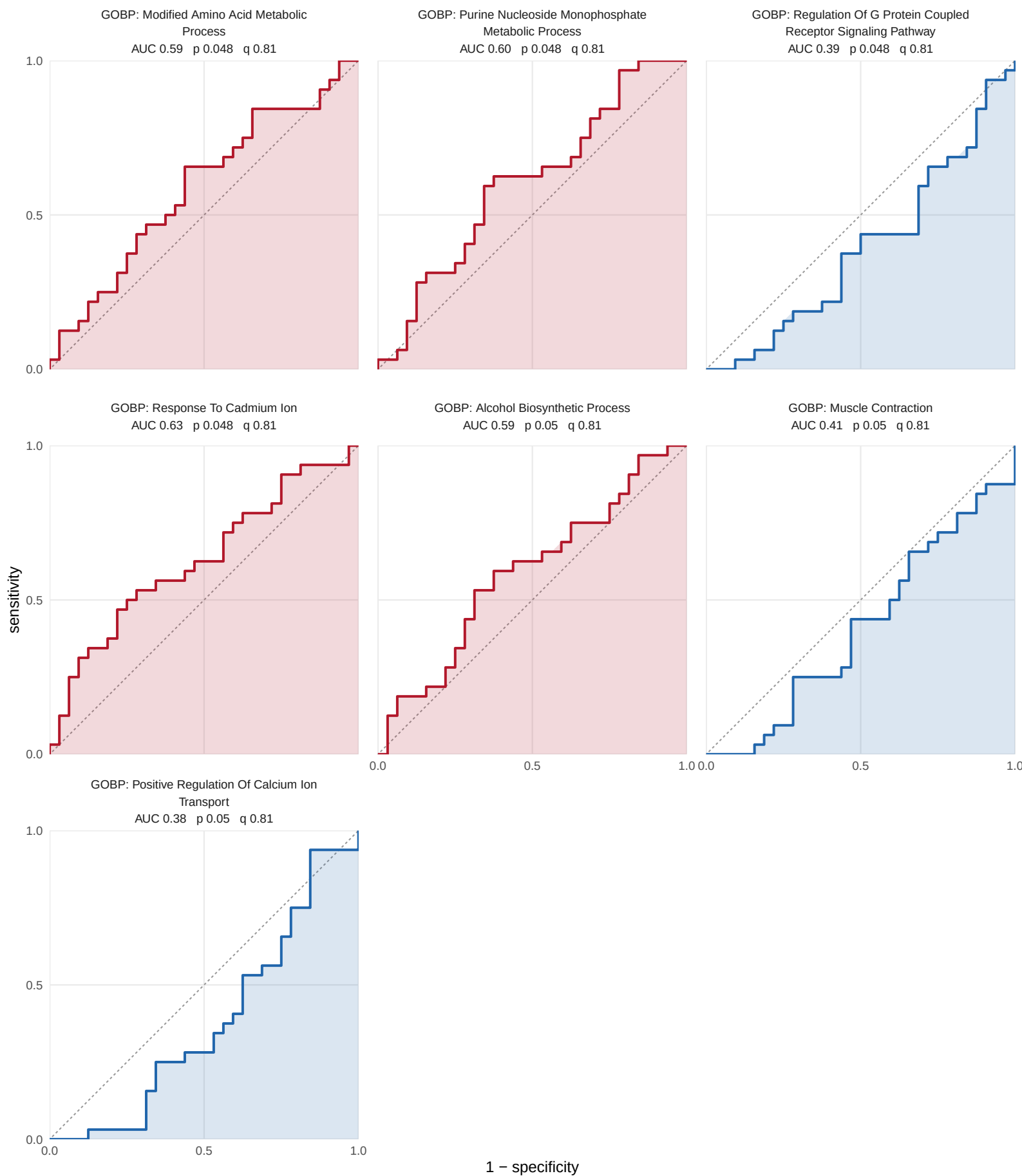
S14 Figure (page 7 of 7). Post BFR vs HLRT, GOBP. ROC curves for all 79 GOBP sets whose sing score separates the groups at nominal p, across 32 paired participants, smallest p first. AUC has its direction fixed: red separates higher in BFR, blue lower. Shading is area under the curve, dashed line chance. p from the paired Wilcoxon signed-rank test, q from BH within collection and task. Nominal p, uncorrected: chance alone returns 68.3 of the 1366 GOBP sets. Data: set_auc sheet of 05_set_classification.xlsx.
