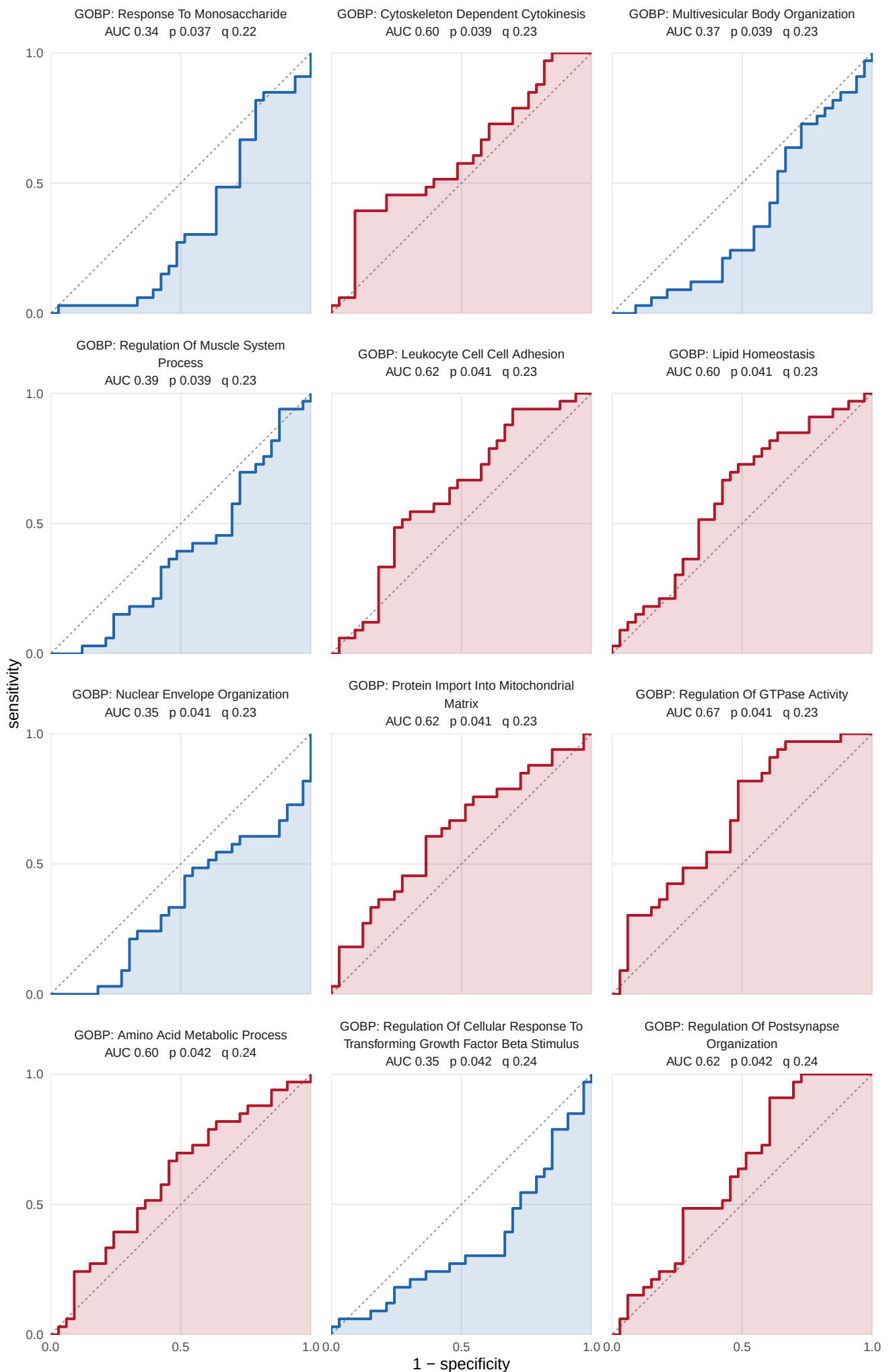
S13 Figure (page 20 of 22). Pre to post, HLRT, GOBP. ROC curves for all 255 GOBP sets whose singscore separates the groups at nominal p, across 33 paired legs, smallest p first. AUC has its direction fixed: red separates higher in post, blue lower. Shading is area under the curve, dashed line chance. p from the paired Wilcoxon signed-rank test, q from BH within collection and task. Nominal p, uncorrected: chance alone returns 68.3 of the 1366 GOBP sets. Data: set_auc sheet of 05_set_classification.xlsx.
