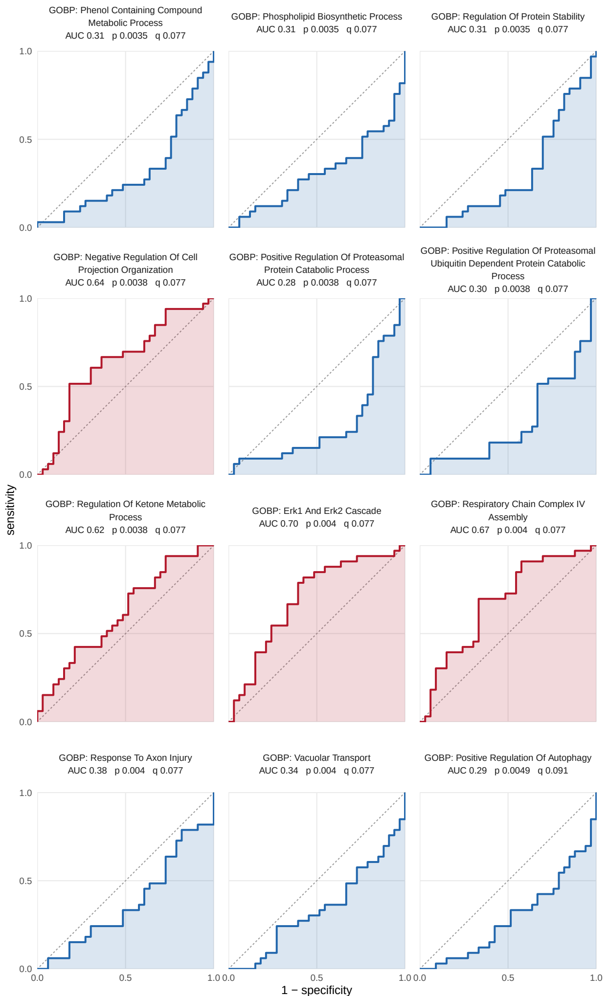
S13 Figure (page 6 of 22). Pre to post, HLRT, GOBP. ROC curves for all 255 GOBP sets whose singscore separates the groups at nominal p, across 33 paired legs, smallest p first. AUC has its direction fixed: red separates higher in post, blue lower. Shading is area under the curve, dashed line chance. p from the paired Wilcoxon signed-rank test, q from BH within collection and task. Nominal p, uncorrected: chance alone returns 68.3 of the 1366 GOBP sets. Data: set_auc sheet of 05_set_classification.xlsx.
