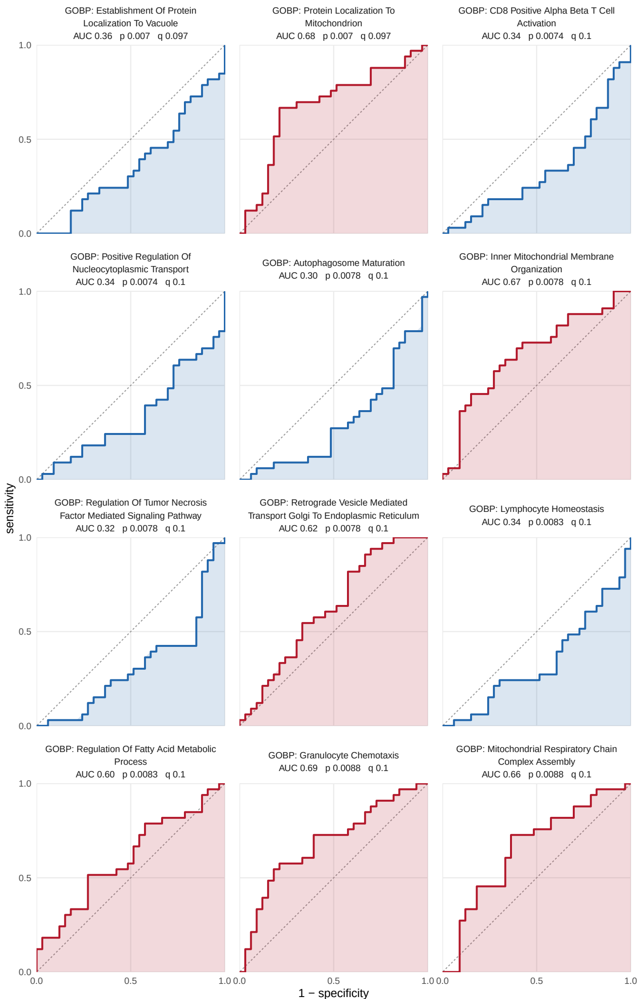
S13 Figure (page 9 of 22). Pre to post, HLRT, GOBP. ROC curves for all 255 GOBP sets whose singscore separates the groups at nominal p, across 33 paired legs, smallest p first. AUC has its direction fixed: red separates higher in post, blue lower. Shading is area under the curve, dashed line chance. p from the paired Wilcoxon signed-rank test, q from BH within collection and task. Nominal p, uncorrected: chance alone returns 68.3 of the 1366 GOBP sets. Data: set_auc sheet of 05_set_classification.xlsx.
