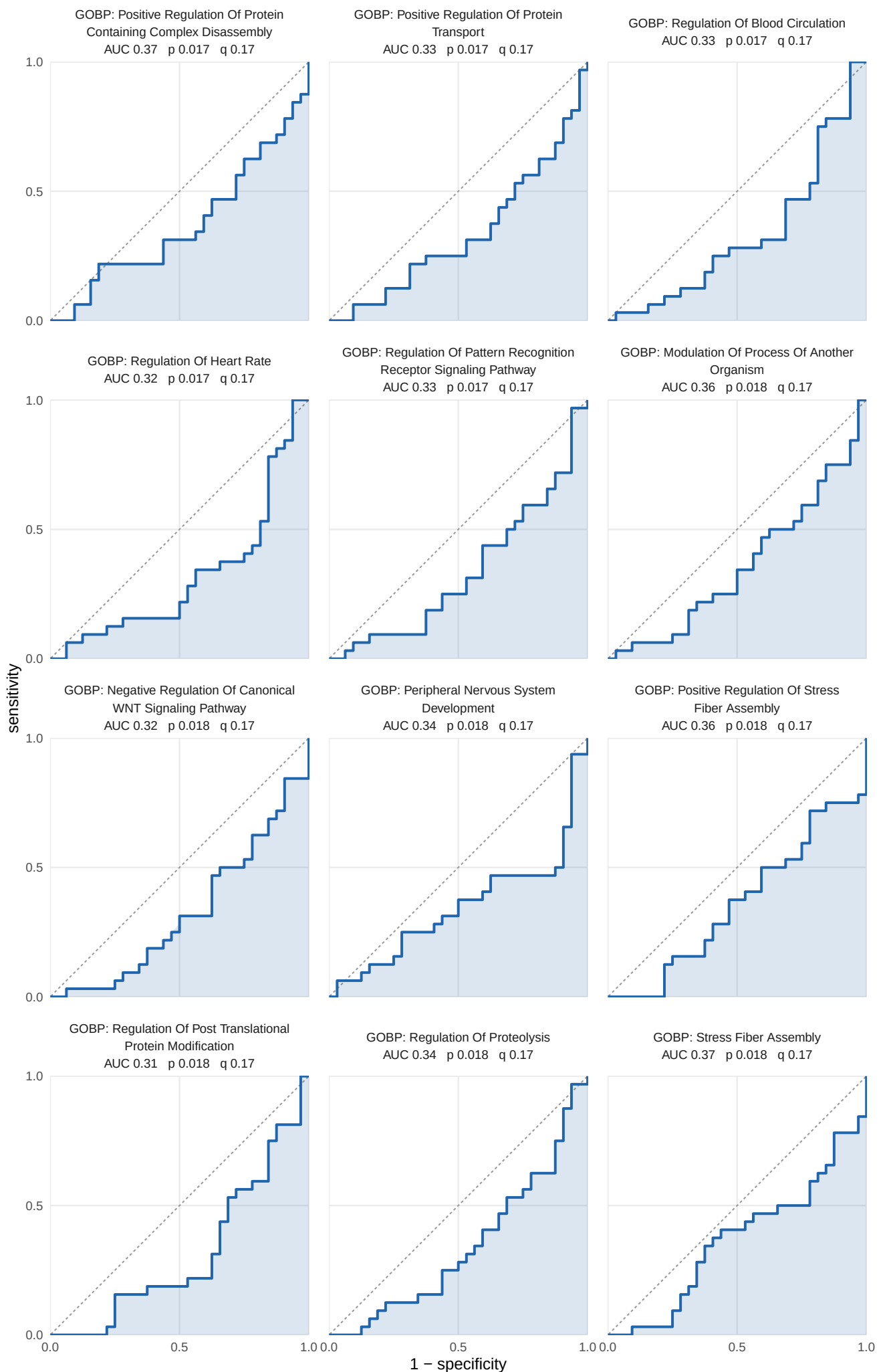
S12 Figure (page 12 of 23). Pre to post, BFR, GOBP. ROC curves for all 274 GOBP sets whose singscore separates the groups at nominal p, across 32 paired legs, smallest p first. AUC has its direction fixed: red separates higher in post, blue lower. Shading is area under the curve, dashed line chance. p from the paired Wilcoxon signed-rank test, q from BH within collection and task. Nominal p, uncorrected: chance alone returns 68.3 of the 1366 GOBP sets. Data: set_auc sheet of 05_set_classification.xlsx.
