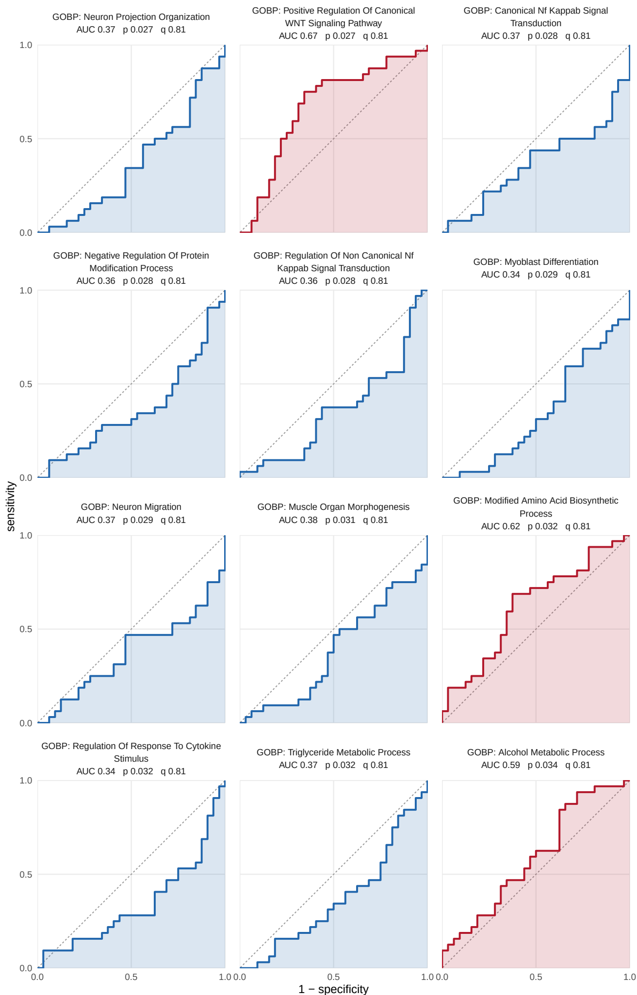
S14 Figure (page 4 of 7). Post BFR vs HLRT, GOBP. ROC curves for all 79 GOBP sets whose singscore separates the groups at nominal p, across 32 paired participants, smallest p first. AUC has its direction fixed: red separates higher in BFR, blue lower. Shading is area under the curve, dashed line chance. p from the paired Wilcoxon signed-rank test, q from BH within collection and task. Nominal p, uncorrected: chance alone returns 68.3 of the 1366 GOBP sets. Data: set_auc sheet of 05_set_classification.xlsx.
