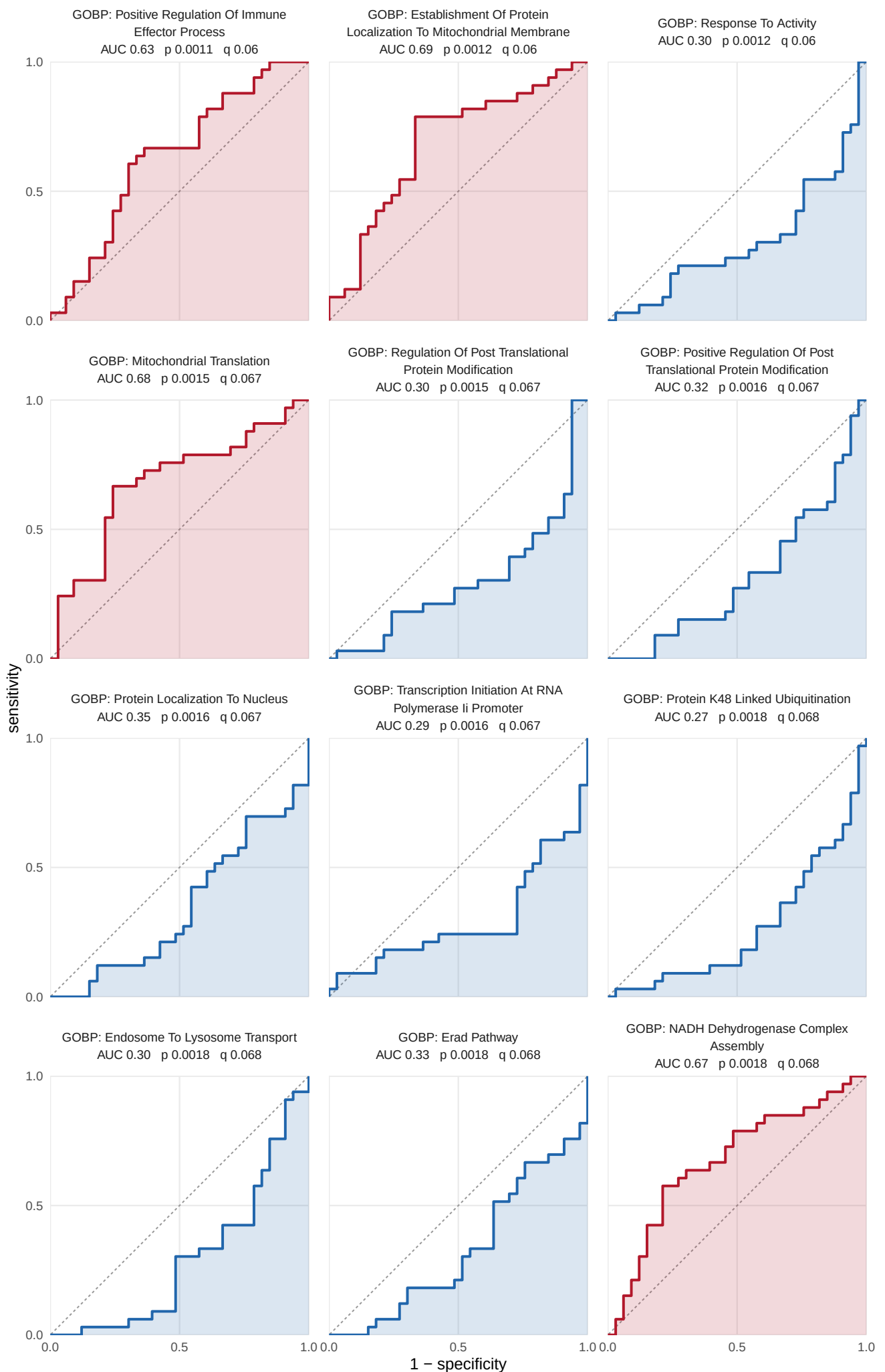
S13 Figure (page 3 of 22). Pre to post, HLRT, GOBP. ROC curves for all 255 GOBP sets whose singscore separates the groups at nominal p, across 33 paired legs, smallest p first. AUC has its direction fixed: red separates higher in post, blue lower. Shading is area under the curve, dashed line chance. p from the paired Wilcoxon signed-rank test, q from BH within collection and task. Nominal p, uncorrected: chance alone returns 68.3 of the 1366 GOBP sets. Data: set_auc sheet of 05_set_classification.xlsx.
