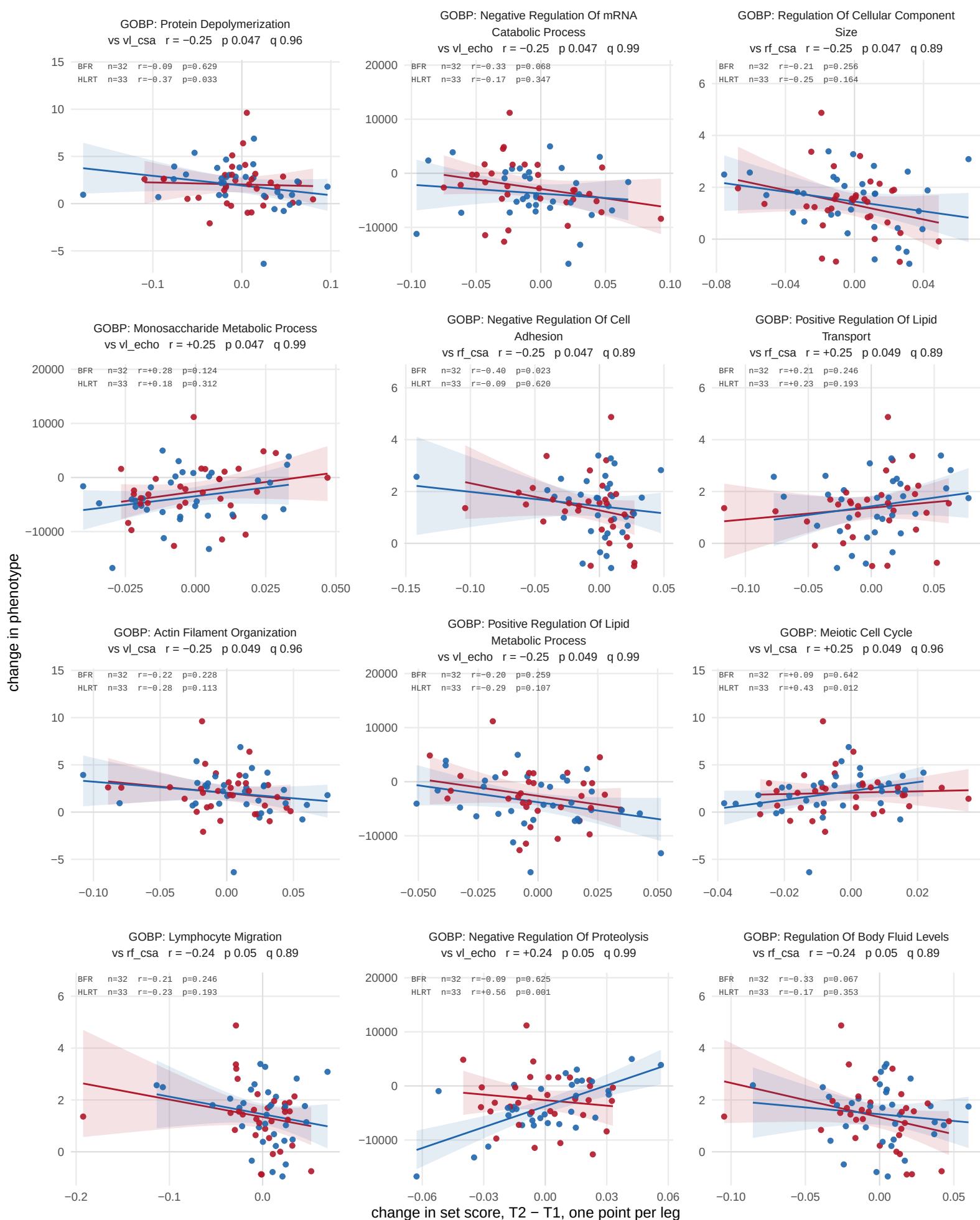
S17 Figure (page 17 of 17). Training response against phenotype, all legs, GOBP. All 204 GOBP set-outcome pairs whose Spearman correlation reaches nominal p in the pooled analysis (65 legs, both arms pooled), smallest p first. Lines are fitted within each arm; the header r is the pooled correlation and the inset gives it within each arm. q from BH within collection and outcome. Nominal p , uncorrected: chance alone returns 68.3 of the 1366 GOBP sets. Data: set_association and set_by_arm sheets of 06_set_association.xlsx.
