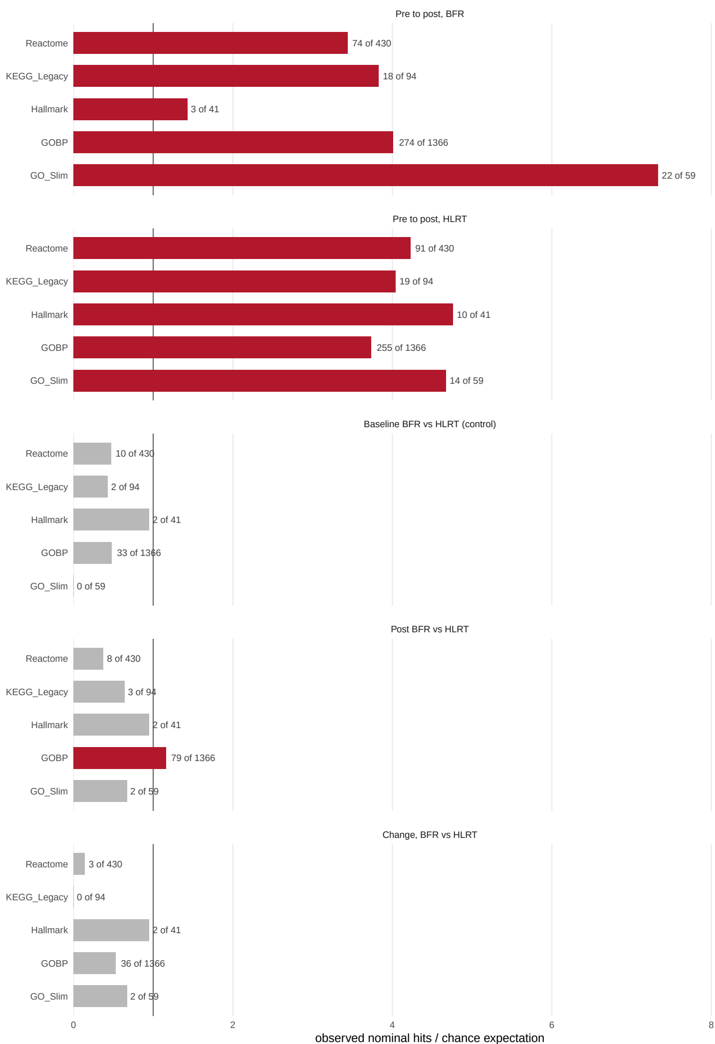
S16 Figure. Nominal hits relative to chance, by collection. Paired Wilcoxon per set across 5 collections, uncorrected p. Bar length is observed nominal hits divided by the count that collection returns under the null; red clears 1, grey does not. Labels give observed of tested. Data: chance_expectation sheet of 05_set_classification.xlsx.
