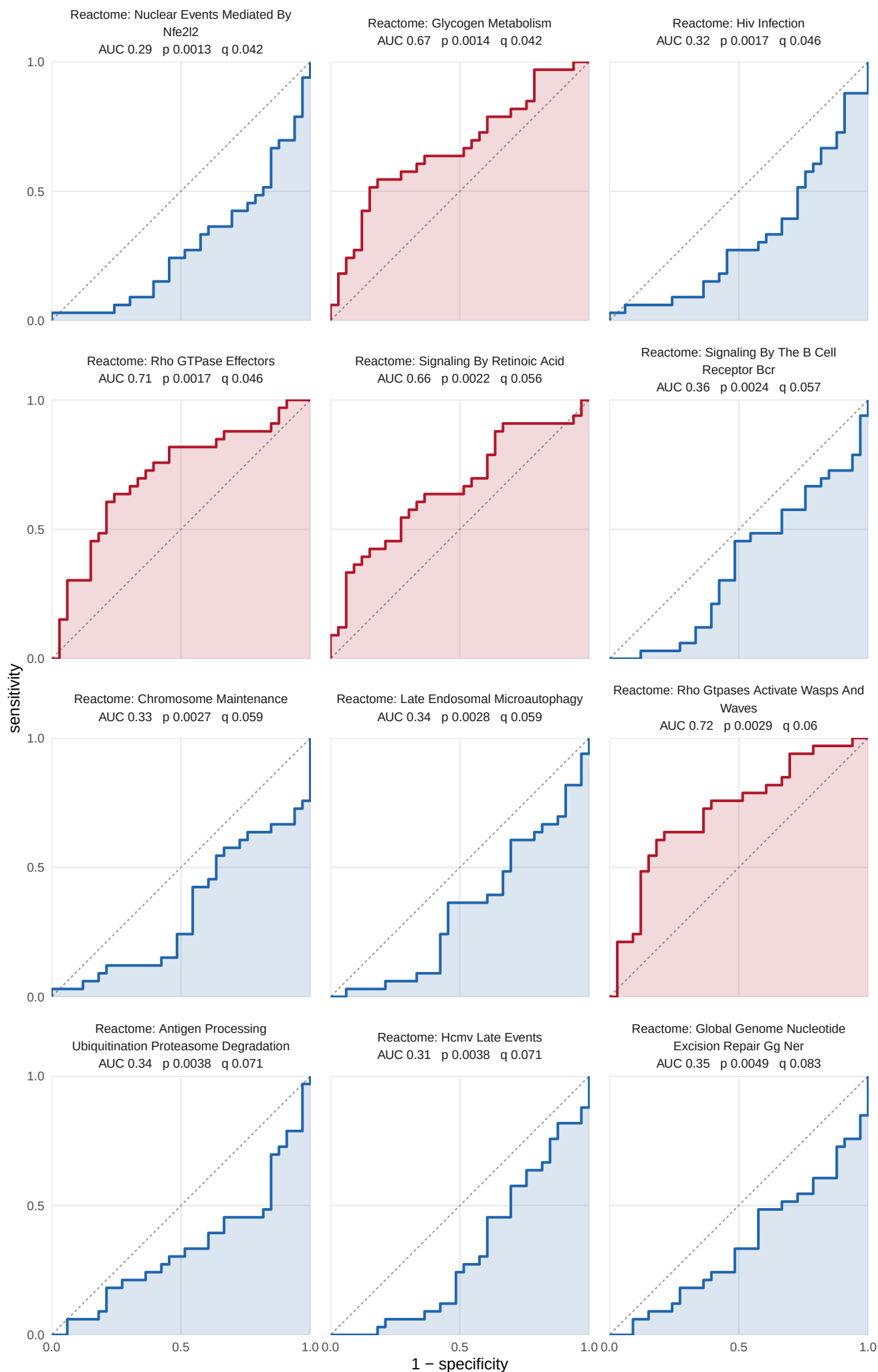
S13 Figure (page 2 of 8). Pre to post, HLRT, Reactome. ROC curves for all 91 Reactome sets whose singscore separates the groups at nominal p, across 33 paired legs, smallest p first. AUC has its direction fixed: red separates higher in post, blue lower. Shading is area under the curve, dashed line chance. p from the paired Wilcoxon signed-rank test, q from BH within collection and task. Nominal p, uncorrected: chance alone returns 21.5 of the 430 Reactome sets. Data: set_auc sheet of 05_set_classification.xlsx.
