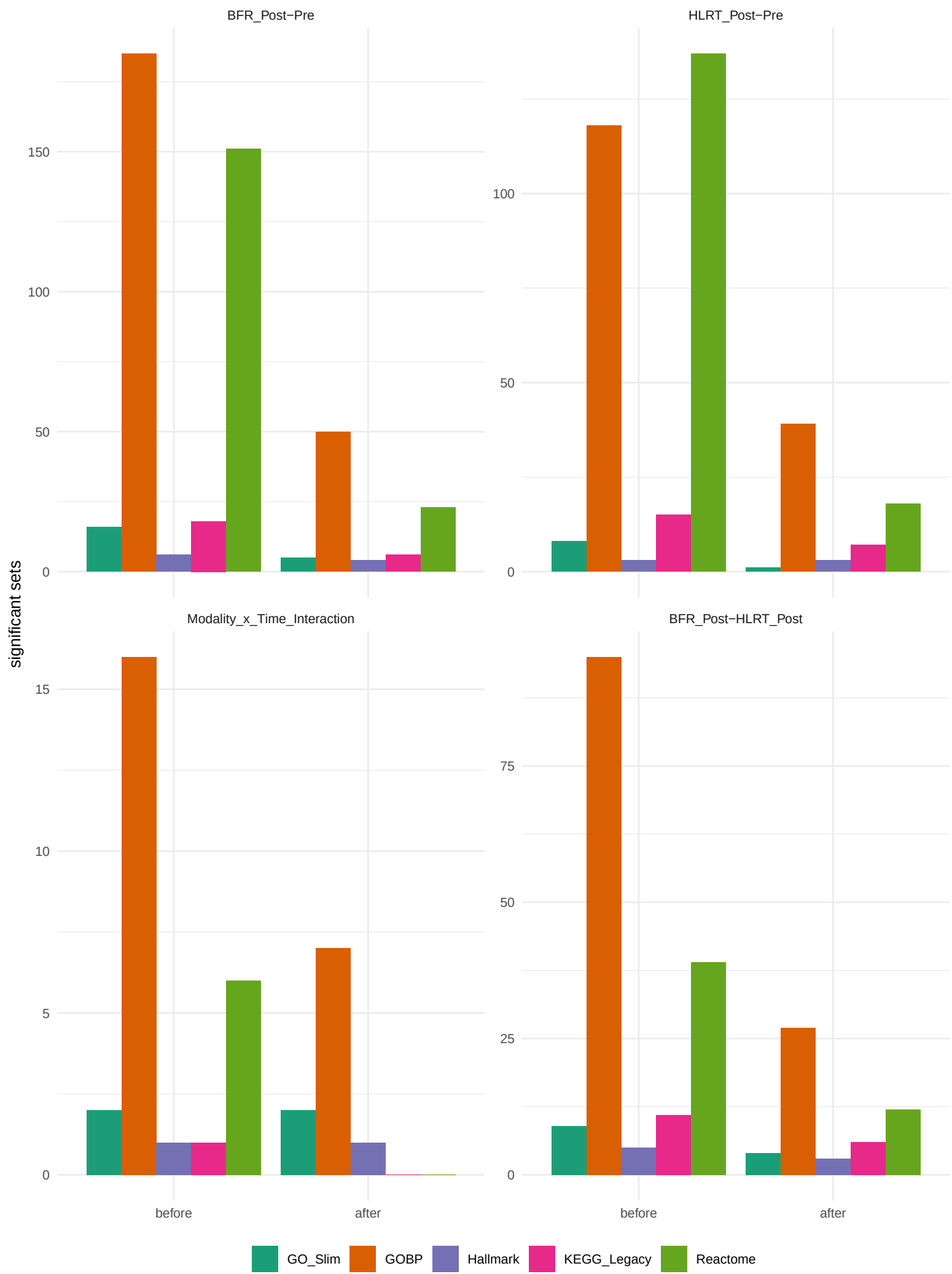
S7 Figure. Significant sets before and after collapse. Sets at FDR 0.05 per collection and contrast, before and after collapsePathways, which keeps a set only if it stands alone given a stronger set's leading edge. Data: set_tests sheet of 01_run_fgsea_and_fry.xlsx.
