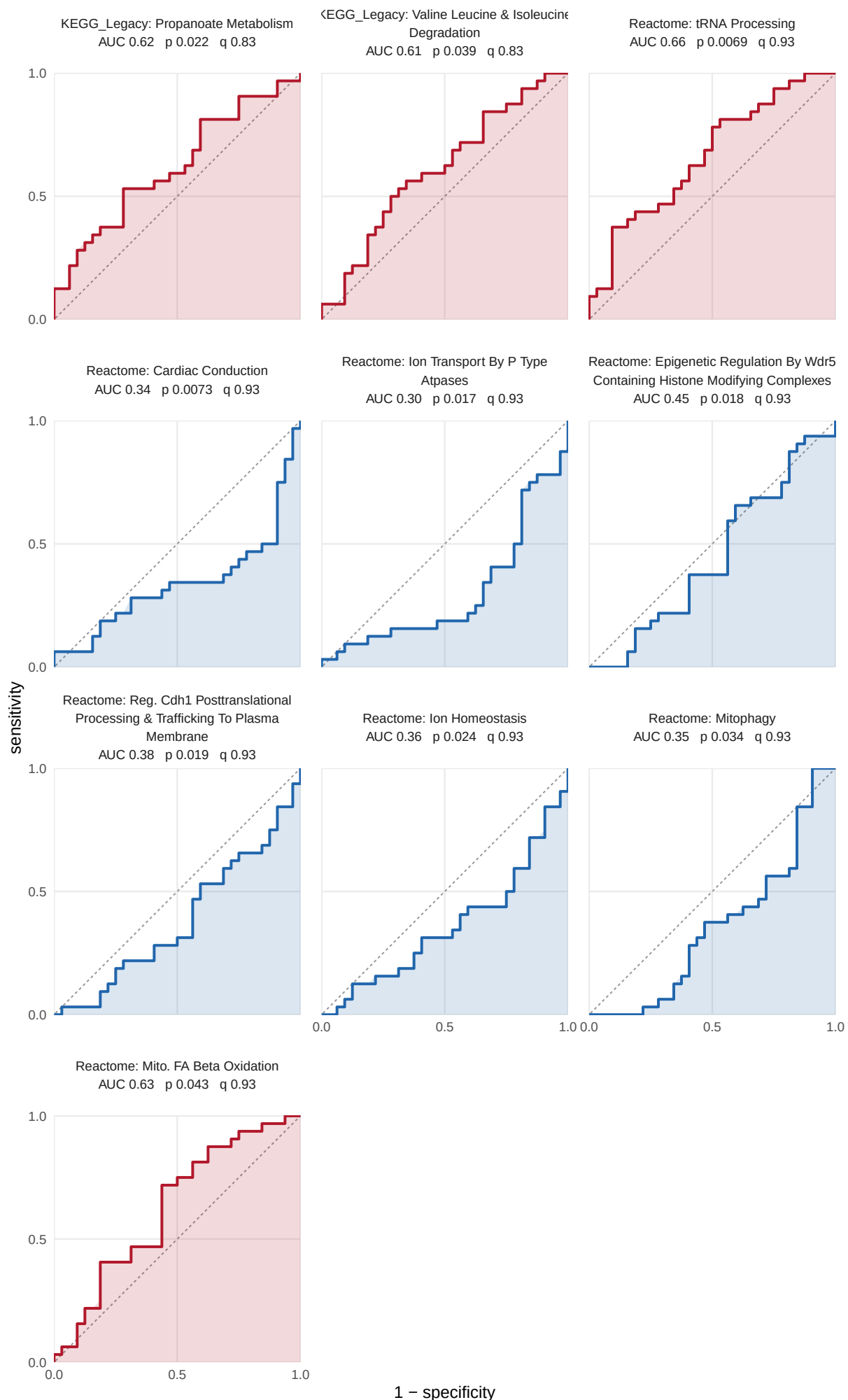
S15 Figure (page 8 of 8). ROC curves for set scores, Post BFR vs HLRT. ROC curves for all 94 sets whose sing score separates the groups at nominal p, across 32 paired participants, by collection then p. AUC has its direction fixed: red separates higher in BFR, blue lower. Shading is area under the curve, dashed line chance. p from the paired Wilcoxon signed-rank test, q from BH within collection and task. Nominal p, uncorrected. Each collection is read against its own expectation: GOBP 68.3 of 1366, GO_Slim 3.0 of 59, Hallmark 2.1 of 41, KEGG_Legacy 4.7 of 94, Reactome 21.5 of 430. Data: set_auc sheet of 05_classify_and_associate_sets.xlsx.
