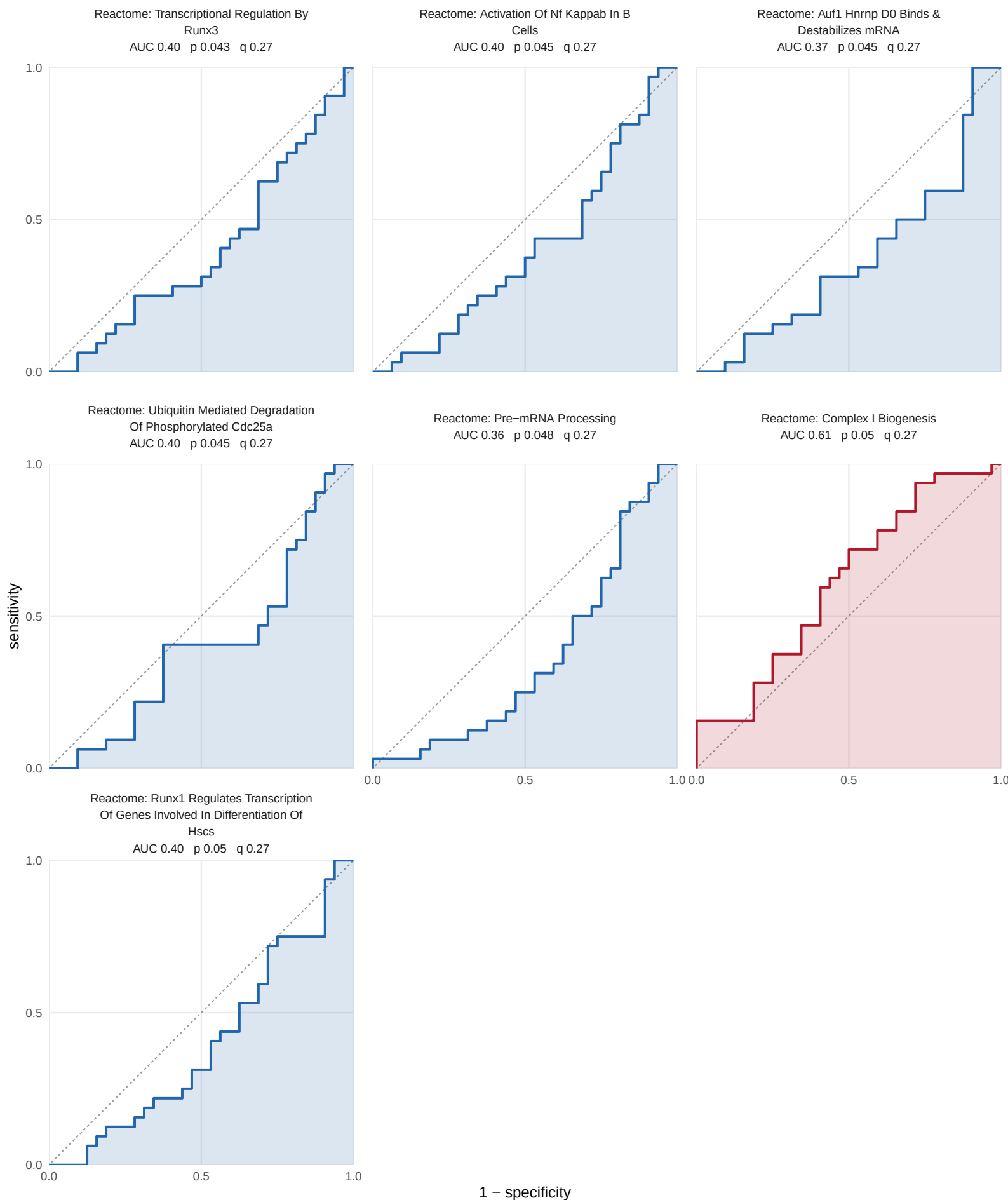
S13 Figure (page 33 of 33). ROC curves for set scores, Pre to post, BFR. ROC curves for all 391 sets whose singscore separates the groups at nominal p, across 32 paired legs, by collection then p. AUC has its direction fixed: red separates higher in post, blue lower. Shading is area under the curve, dashed line chance. p from the paired Wilcoxon signed-rank test, q from BH within collection and task. Nominal p, uncorrected. Each collection is read against its own expectation: GOBP 68.3 of 1366, GO_Slim 3.0 of 59, Hallmark 2.1 of 41, KEGG_Legacy 4.7 of 94, Reactome 21.5 of 430. Data: set_auc sheet of 05_classify_and_associate_sets.xlsx.
