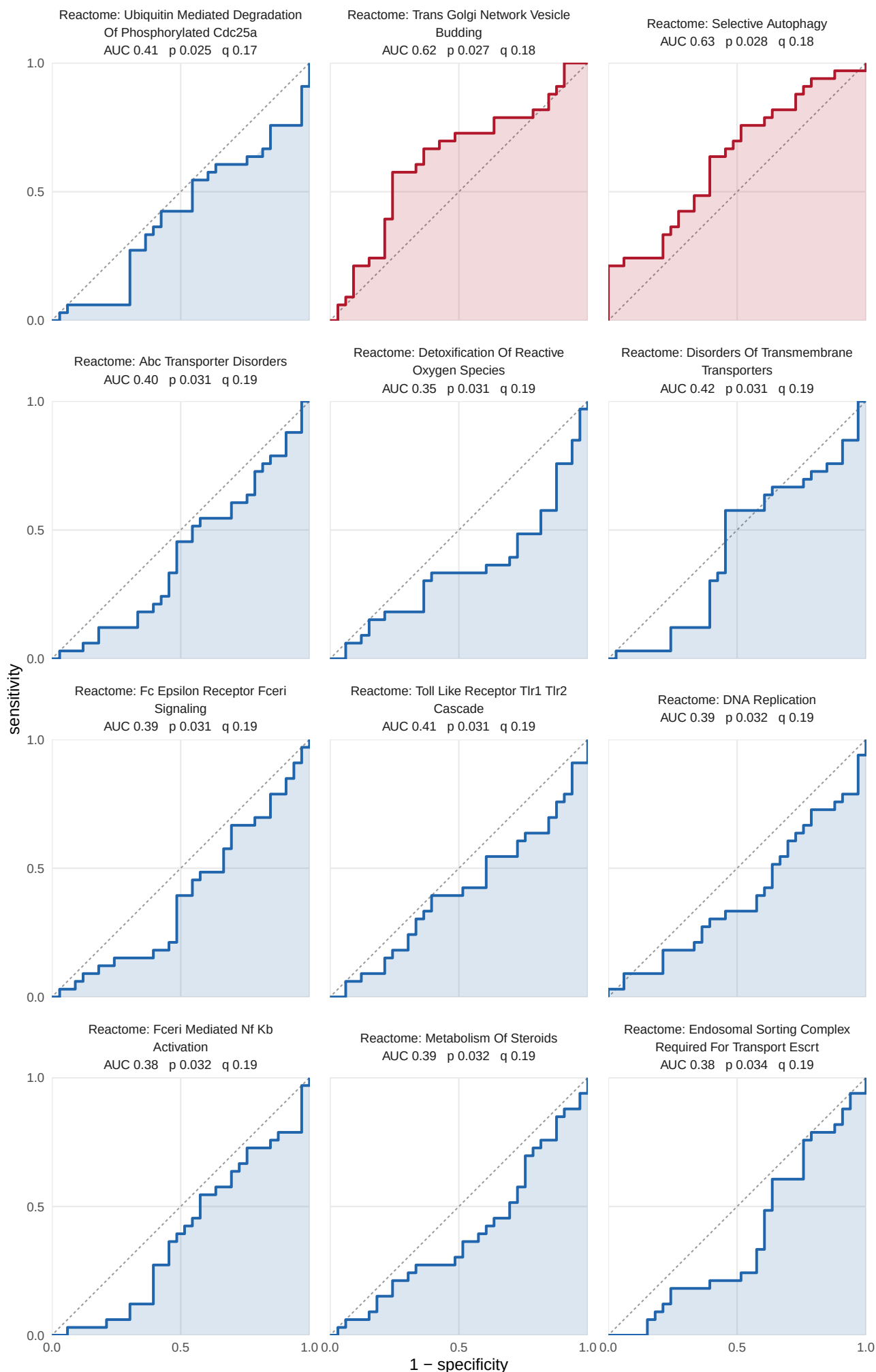
S14 Figure (page 31 of 33). ROC curves for set scores, Pre to post, HLRT. ROC curves for all 389 sets whose singscore separates the groups at nominal p, across 33 paired legs, by collection then p. AUC has its direction fixed: red separates higher in post, blue lower. Shading is area under the curve, dashed line chance. p from the paired Wilcoxon signed-rank test, q from BH within collection and task. Nominal p, uncorrected. Each collection is read against its own expectation: GOBP 68.3 of 1366, GO_Slim 3.0 of 59, Hallmark 2.1 of 41, KEGG_Legacy 4.7 of 94, Reactome 21.5 of 430. Data: set_auc sheet of 05_classify_and_associate_sets.xlsx.
