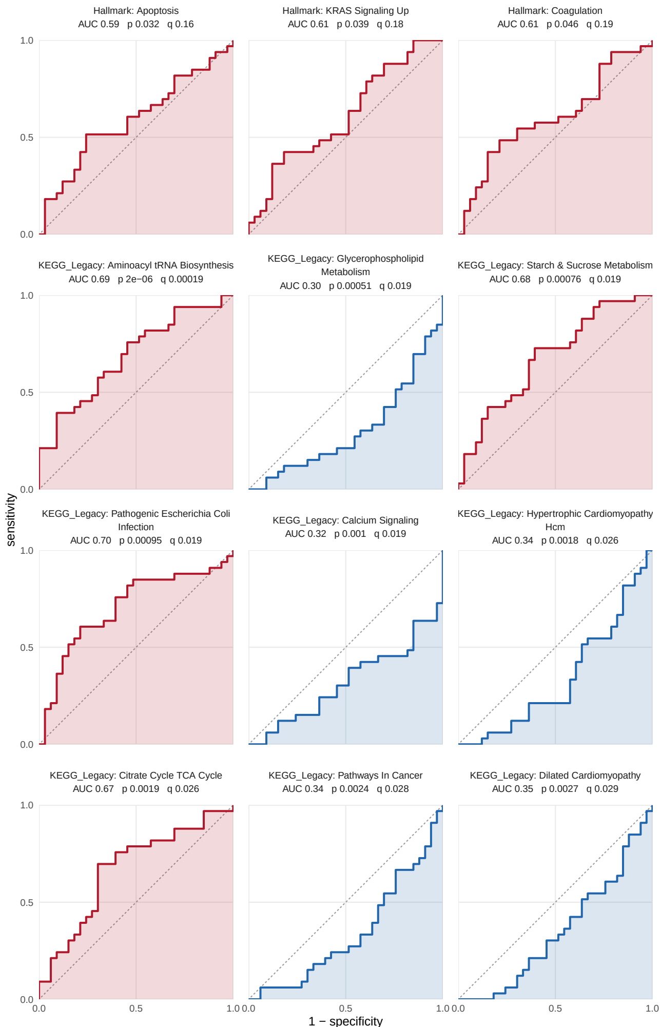
S14 Figure (page 24 of 33). ROC curves for set scores, Pre to post, HLRT. ROC curves for all 389 sets whose singscore separates the groups at nominal p, across 33 paired legs, by collection then p. AUC has its direction fixed: red separates higher in post, blue lower. Shading is area under the curve, dashed line chance. p from the paired Wilcoxon signed-rank test, q from BH within collection and task. Nominal p, uncorrected. Each collection is read against its own expectation: GOBP 68.3 of 1366, GO_Slim 3.0 of 59, Hallmark 2.1 of 41, KEGG_Legacy 4.7 of 94, Reactome 21.5 of 430. Data: set_auc sheet of 05_classify_and_associate_sets.xlsx.
