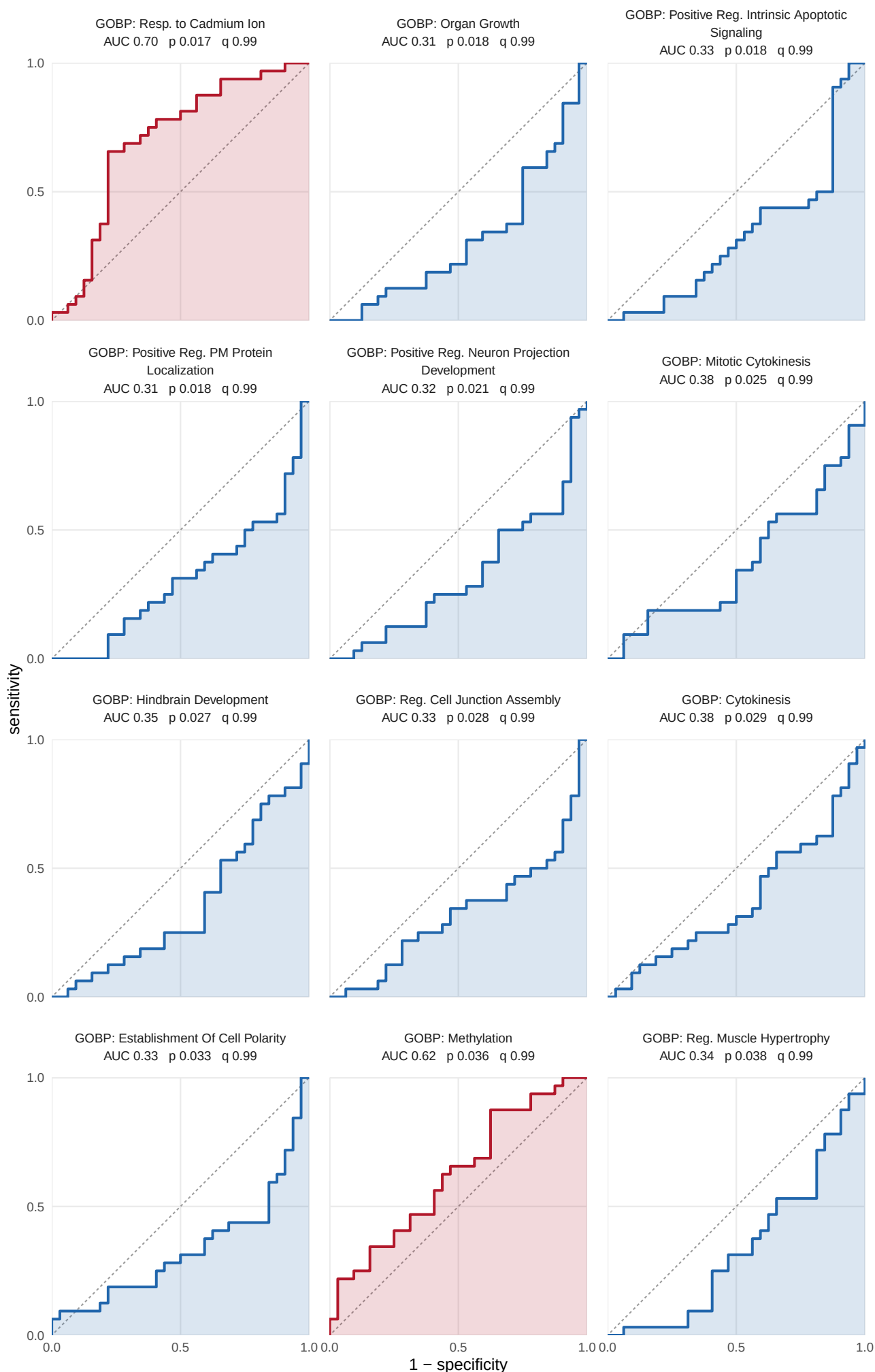
S16 Figure (page 2 of 4). ROC curves for set scores, Change, BFR vs HLRT. ROC curves for all 43 sets whose singscore separates the groups at nominal p, across 32 paired participants, by collection then p. AUC has its direction fixed: red separates higher in BFR, blue lower. Shading is area under the curve, dashed line chance. p from the paired Wilcoxon signed-rank test, q from BH within collection and task. Nominal p, uncorrected. Each collection is read against its own expectation: GOBP 68.3 of 1366, GO_Slim 3.0 of 59, Hallmark 2.1 of 41, KEGG_Legacy 4.7 of 94, Reactome 21.5 of 430. Data: set_auc sheet of 05_classify_and_associate_sets.xlsx.
