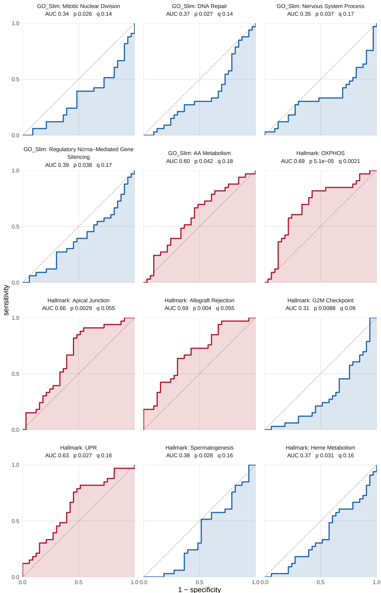
S14 Figure (page 23 of 33). ROC curves for set scores, Pre to post, HLRT. ROC curves for all 389 sets whose sing score separates the groups at nominal p, across 33 paired legs, by collection then p. AUC has its direction fixed: red separates higher in post, blue lower. Shading is area under the curve, dashed line chance. p from the paired Wilcoxon signed-rank test, q from BH within collection and task. Nominal p, uncorrected. Each collection is read against its own expectation: GOBP 68.3 of 1366, GO_Slim 3.0 of 59, Hallmark 2.1 of 41, KEGG_Legacy 4.7 of 94, Reactome 21.5 of 430. Data: set_auc sheet of 05_classify_and_associate_sets.xlsx.
