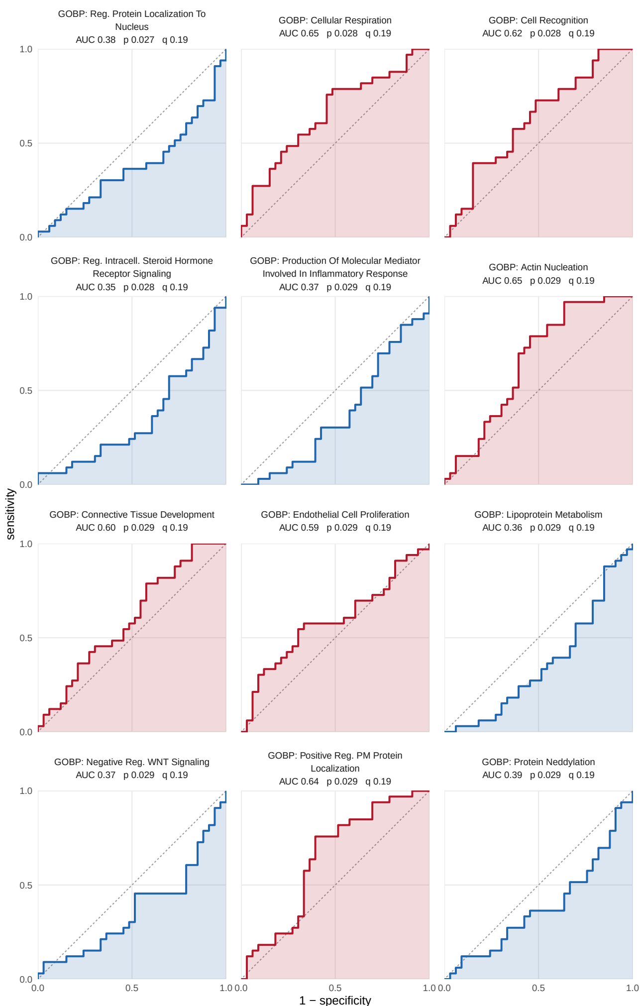
S14 Figure (page 17 of 33). ROC curves for set scores, Pre to post, HLRT. ROC curves for all 389 sets whose singscore separates the groups at nominal p, across 33 paired legs, by collection then p. AUC has its direction fixed: red separates higher in post, blue lower. Shading is area under the curve, dashed line chance. p from the paired Wilcoxon signed-rank test, q from BH within collection and task. Nominal p, uncorrected. Each collection is read against its own expectation: GOBP 68.3 of 1366, GO_Slim 3.0 of 59, Hallmark 2.1 of 41, KEGG_Legacy 4.7 of 94, Reactome 21.5 of 430. Data: set_auc sheet of 05_classify_and_associate_sets.xlsx.
