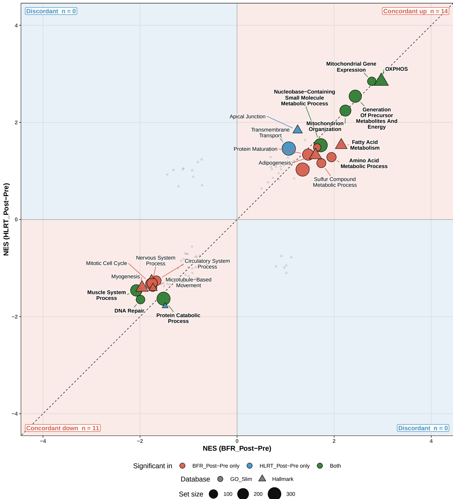
S10 Figure. NES concordance, Hallmark and GO Slim. fgsea NES for the 100 Hallmark and GO Slim sets in BFR_Post-Pre (x) against HLRT_Post-Pre (y). These two collections do not nest, so no branch of the GO:BP hierarchy weights \rho . Grey sets reach neither threshold; coloured ones are significant ( BH < 0.05 within contrast) in one or both. Shaded quadrants move the same way in both contrasts, with their counts in the corners; dashed line is identity. The subtitle gives Spearman's \rho . Data: nes_scatter sheet of 03_enrich_scatter_fgsea.xlsx.
