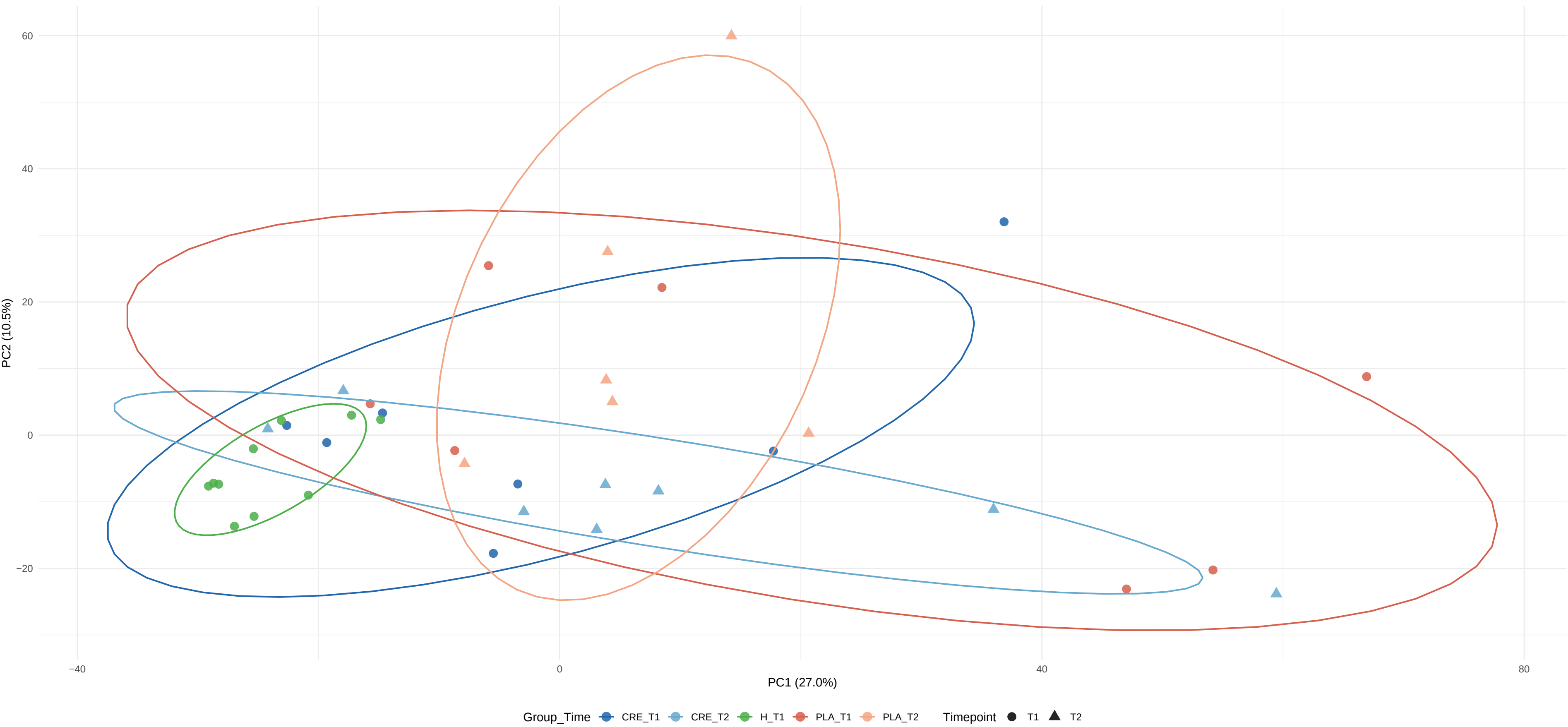
Post-normalization PCA
