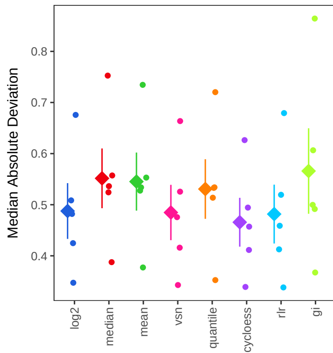
Log2 ratio
