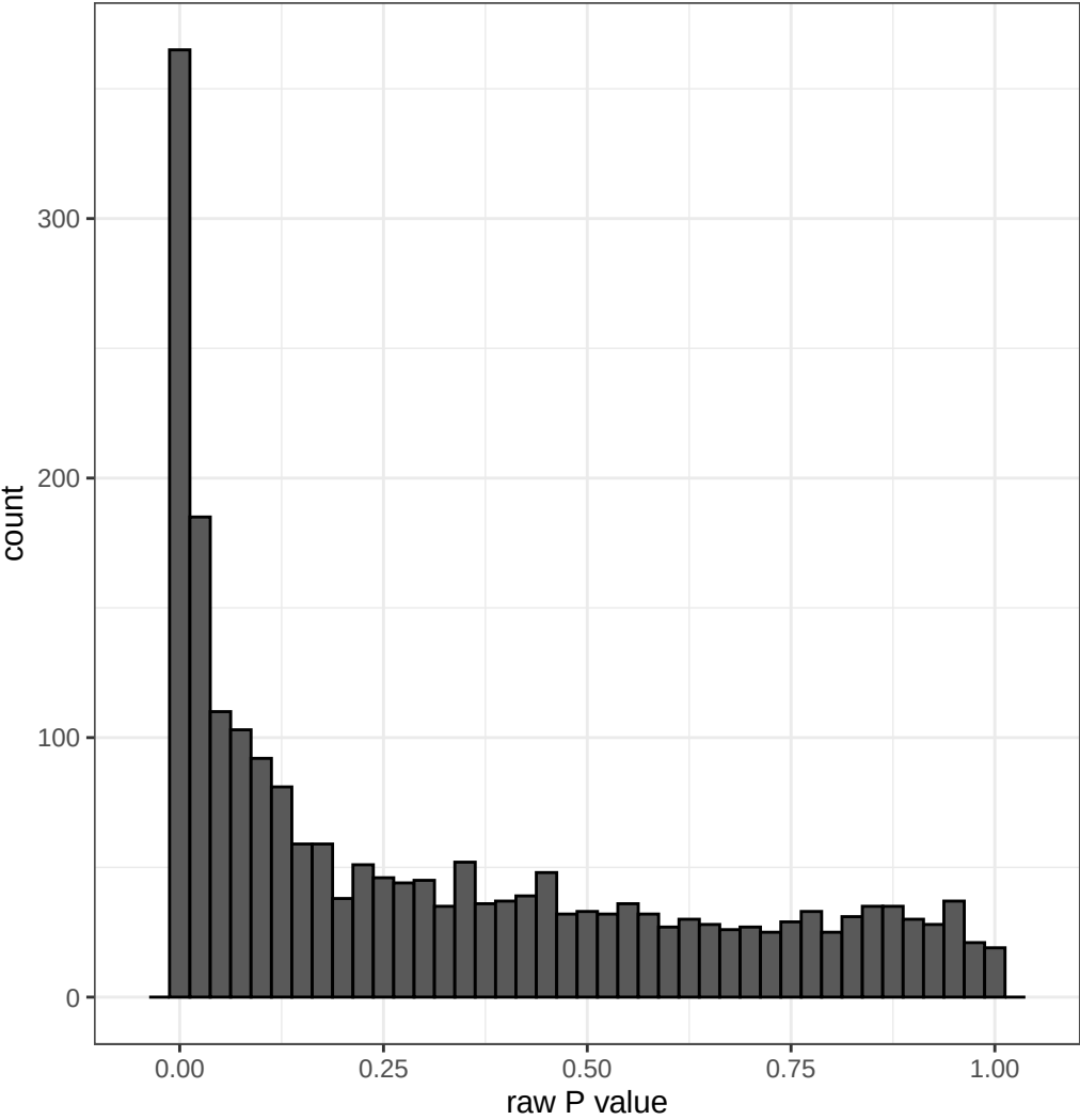
Resid
