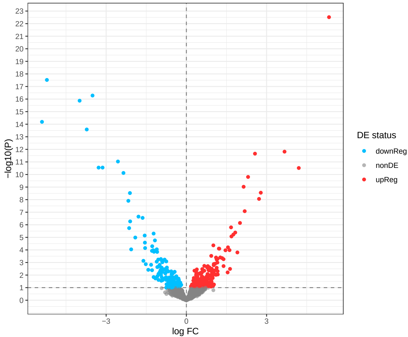
CR_Training, raw p-value
