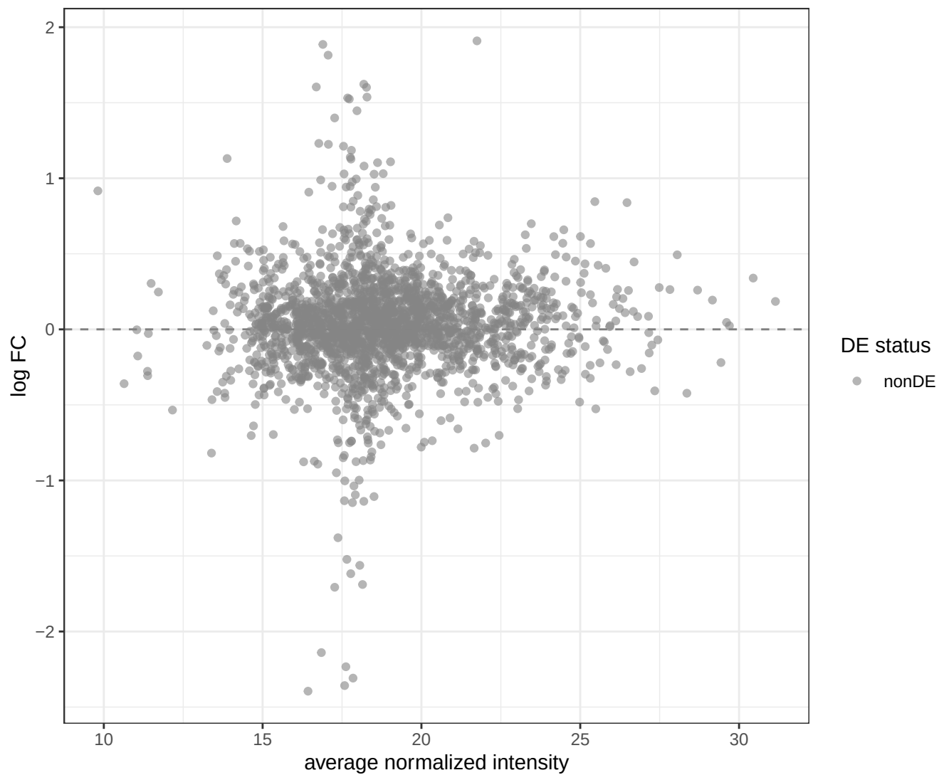
CR_Training, adjusted p-value
