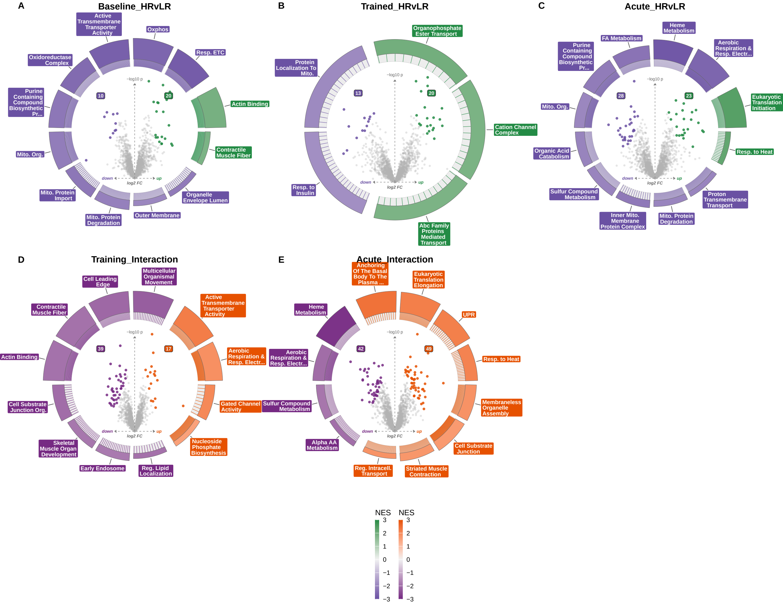
F03 · Where high and low responders differ: pathway enrichment on the volcano Between-responder contrasts (A–C) and the differential-response interactions (D–E). Arcs are fgsea BH q; points are pi-gated. Nothing survives FDR.
