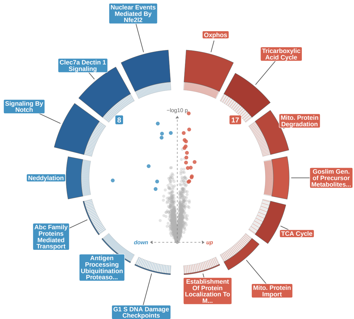
Training_LR
